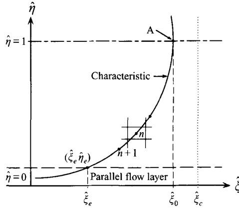
FIGURE 4. Schematic of integration along a characteristic \hat{x}_I = \text{constant} at time t_I : ———, characteristic \hat{x}_I = \hat{\xi}_e ; ·····, current location of fluid particles at time t_I which originated at t_I = -1 on the characteristic curve.
