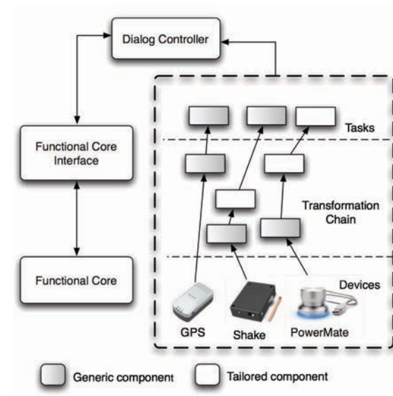
Figure 2. The OI model within an ARCH software architecture.
