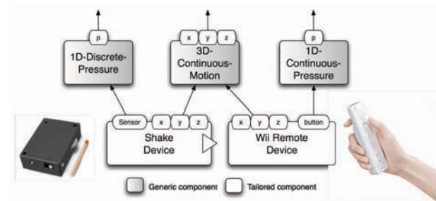
Figure 3. Device components: Shake and Wiimote devices.
