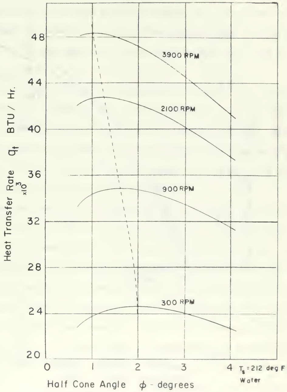
Figure 7. Condensing Limit Heat Transfer Rate vs Half Cone Angle
