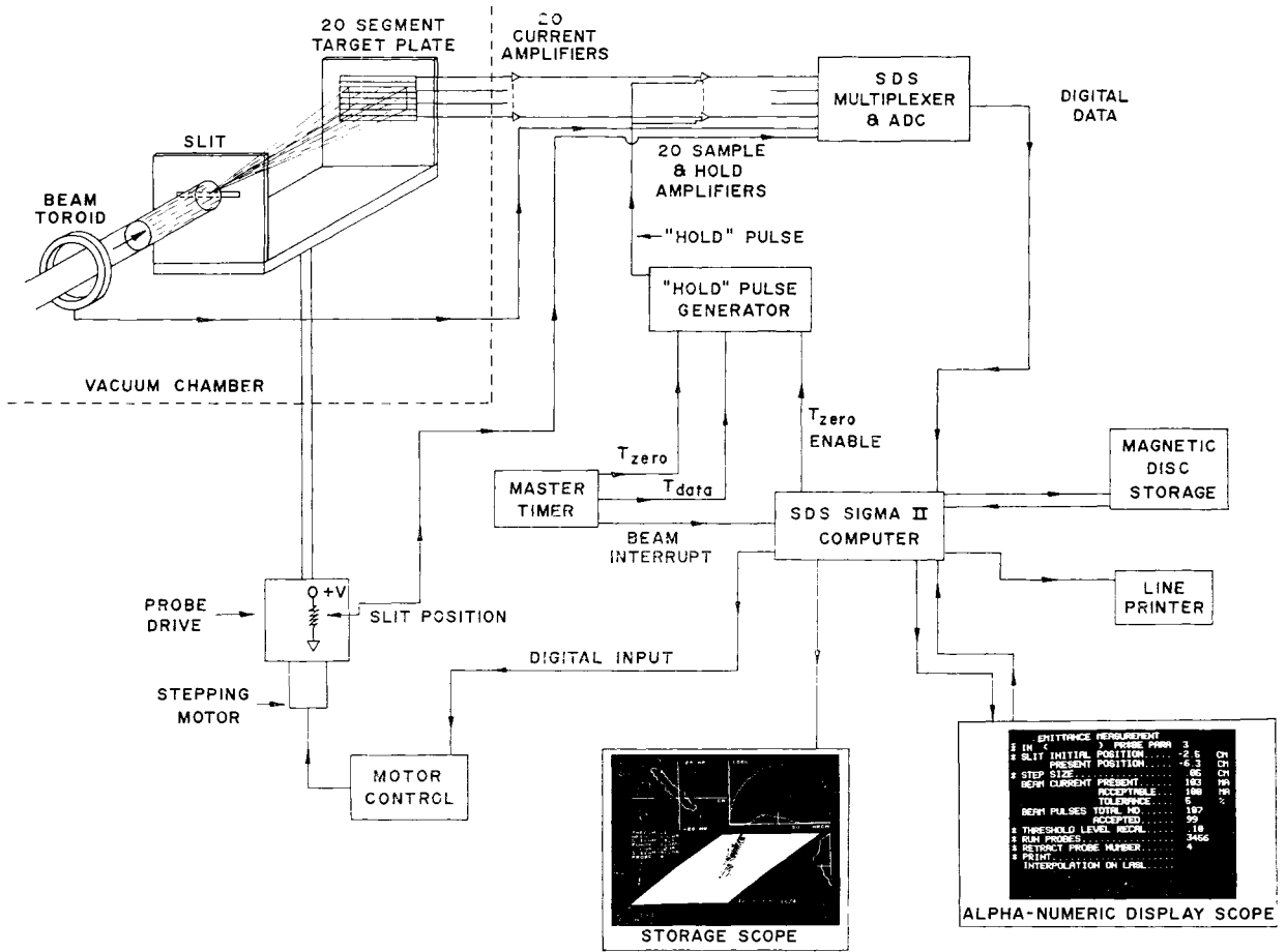
FIG. 10. Emittance measuring equipment.
