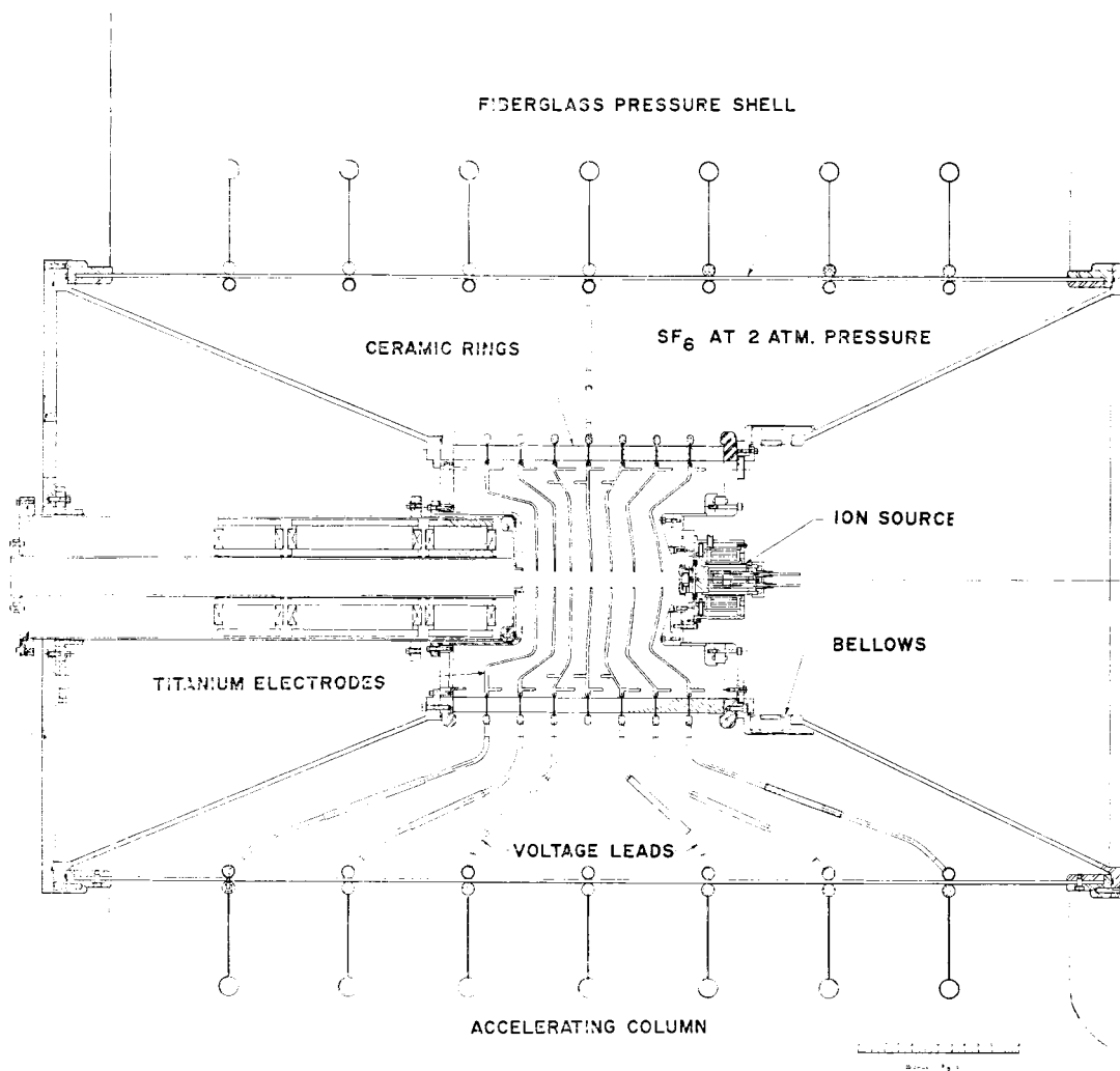
FIG. 2. Accelerator column and ion source.
