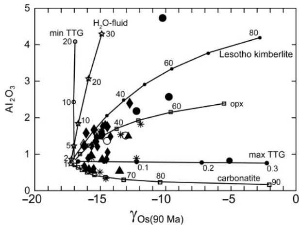
Fig. 12. \gamma_{Os}(90 \text{ Ma}) vs whole-rock \text{Al}_2\text{O}_3 content (wt%) of the Kimberley xenoliths. The lines indicate mixing lines between a strongly depleted mantle end-member and various fluids and melts (compositions are listed in Electronic Appendix Table B1). Mixing is calculated at 90 Ma. Labels on the curves indicate amount of metasomatic component added in per cent. Symbols are as in Fig. 2.
