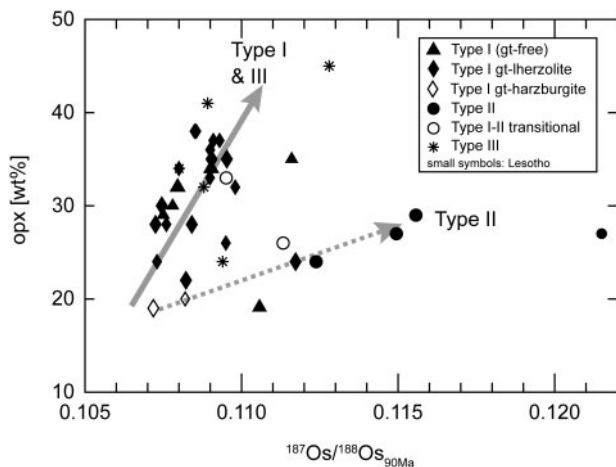
Fig. 13. Correlation of calculated modal orthopyroxene content with ^{187}\text{Os}/^{188}\text{Os}_{90\text{Ma}} of the whole-rocks at 90 Ma.
