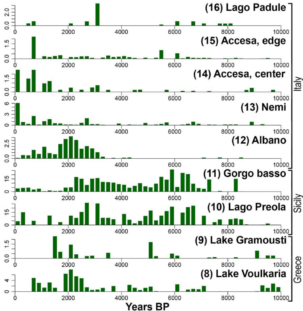
Figure 4. Olea pollen percentages during the Holocene in the Central Mediterranean. Note the different percentage of vertical scales.
