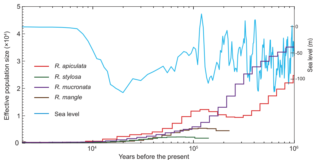
Figure 5. Rhizophora mangrove demography. Historical effective population size ( N_e , y-axis) changes going back in time (x-axis). The changes in N_e are inferred using the PSMC method [48], which relies on the varying level of genetic diversity in different DNA segments across the genome as a basis for the inference of historical N_e changes. In this graph, the generation time ( g ) is set to 20 years and the mutation rate ( \mu ) is 1.6 \times 10^{-8} /bp/generation. Historical sea-level fluctuations are plotted for comparison (blue line) [50].
