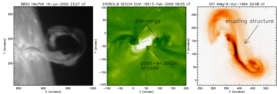
Fig. 2 Lower coronal signatures of the occurrence of a coronal mass ejection (CME). There are a variety of observational manifestations of CMEs including filament eruptions ( left panel ), post-eruption arcades (also called flare arcades, middle panel ), dimming regions ( middle panel ) and rising EUV/soft X-ray structures ( right panel )
