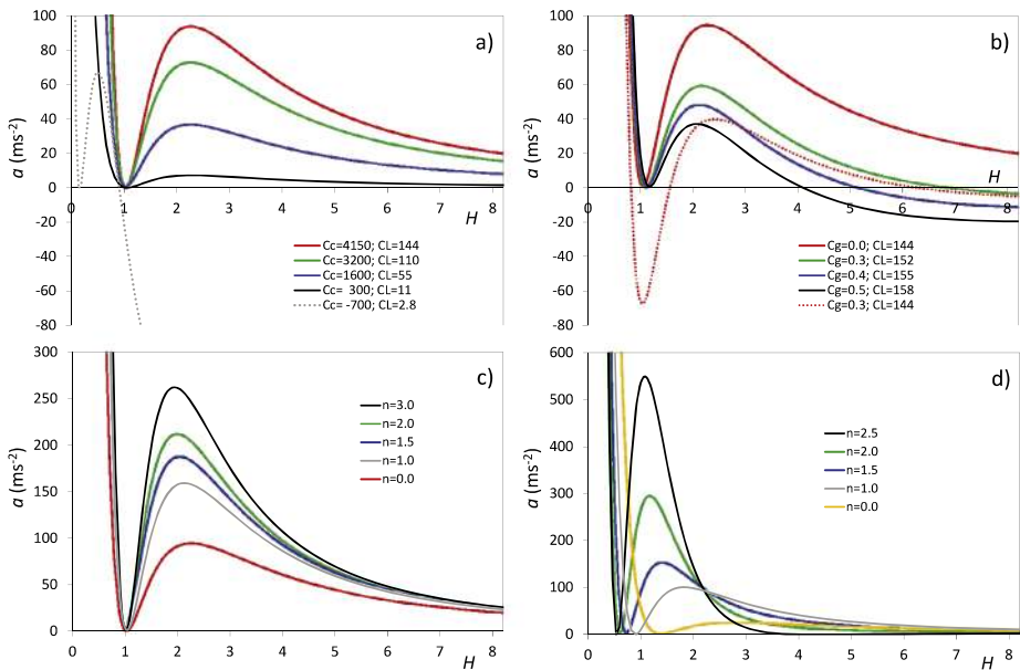
Fig. 7 Flux ropes in the loss-of-equilibrium state: a ) a(H) solutions for different levels of the background-field effect (values of C_c expressed in \text{m s}^{-2} are written in the legend, together with the corresponding critical values of C_L^* ); gray-dotted line represents Kippenhahn–Schlüter configuration with C_g = 1 ( IB_c < 0 , i.e., C_c < 0 ). b ) The gravity effect (values of C_g are written in the legend, together with the corresponding critical values of C_L^* ) calculated using d = 70 Mm, X = 5 , and C_c = 13000 \text{ m s}^{-2} . c ) The effect of decreasing background field (values of the decay index n are given in the legend), calculated using X = 5 , C_L^* = 144 \text{ m s}^{-2} , C_c = 13000 \text{ m s}^{-2} , and C_g = 0 . d ) The torus-instability effect (values of n are given in the legend), calculated using the same set of parameters as in c )
