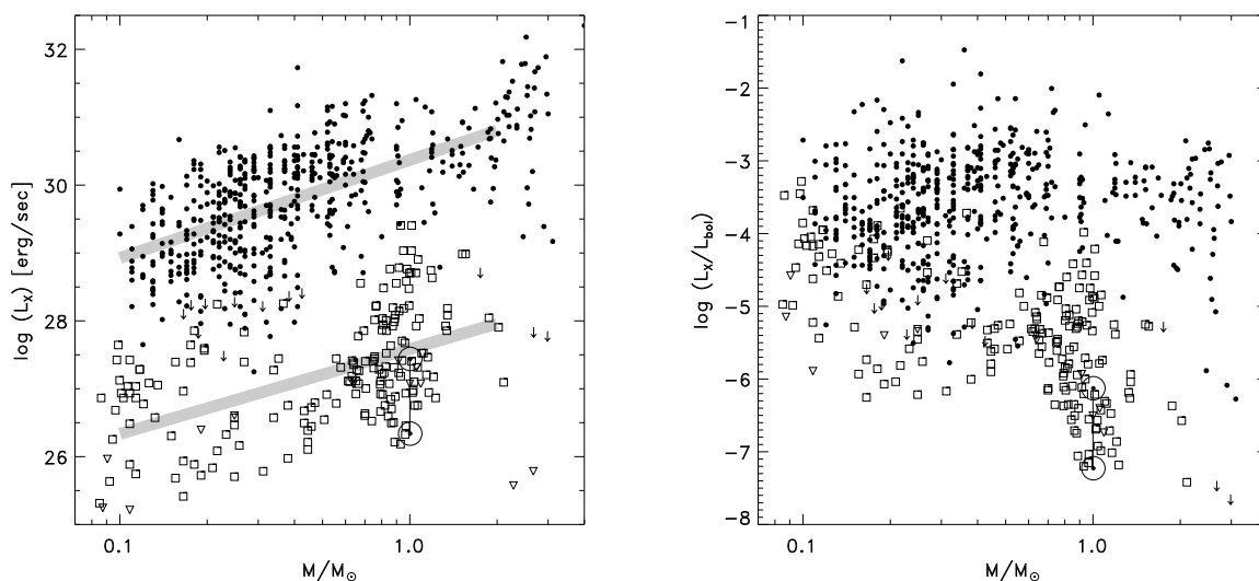
Fig. 7.— Absolute (left) and fractional (right) X-ray luminosity versus stellar mass for the stars in the COUP optical sample (solid dots, arrows for upper limits) based on masses determined with the PMS models of Siess, Dufour, & Forestini (2000), and for the NEXXUS sample of nearby field stars (open squares, triangles for upper limits). The thick grey lines in the L_X \leftrightarrow M correlation show the linear regression fits with the EM algorithm in ASURV for the low-mass ( M \leq 2 M_\odot ) stars in these two samples.
