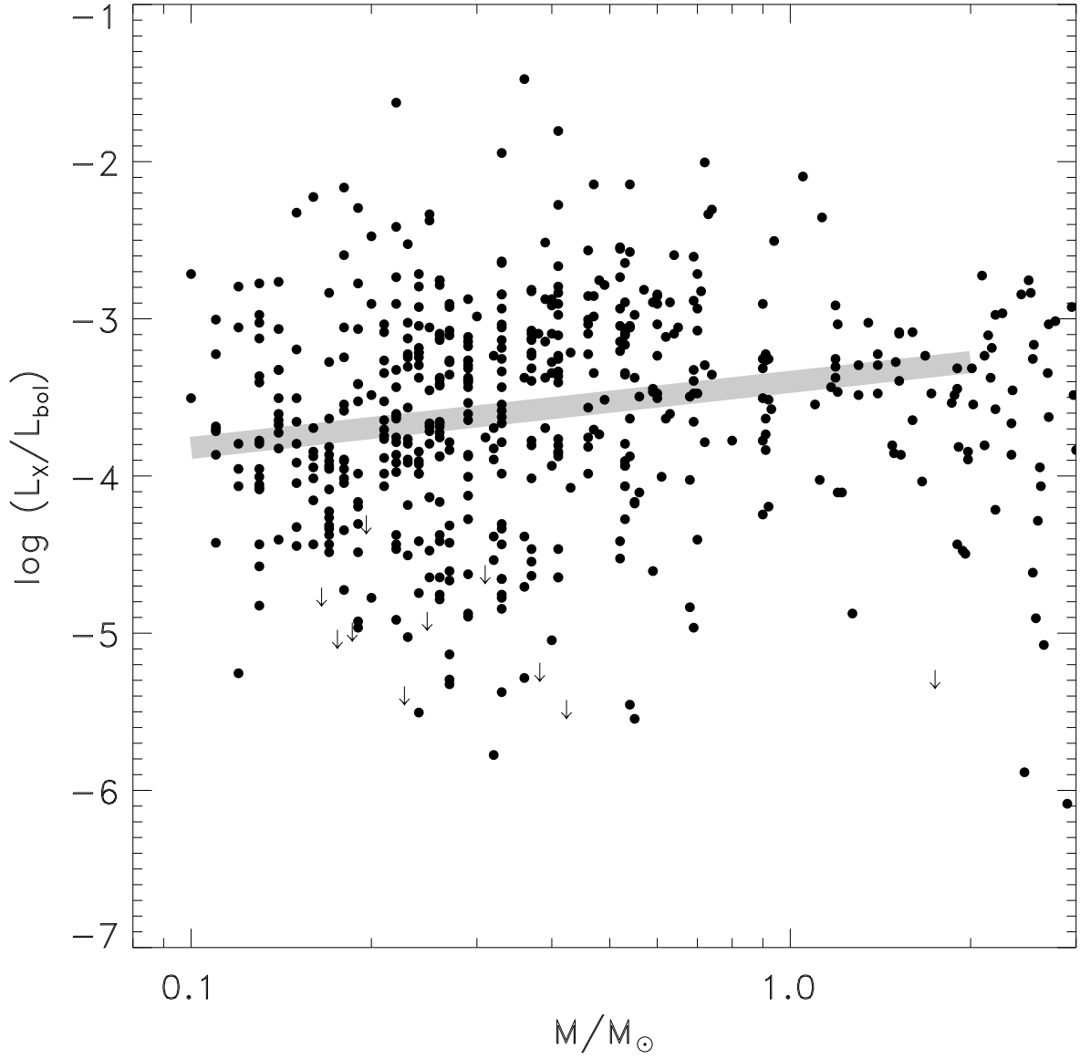
Fig. 4.— Fractional X-ray luminosity versus stellar mass for the low-mass stars in the COUP optical sample. The line shows the linear regression fit for the low-mass stars ( M \leq 2 M_\odot ) with the EM algorithm computed with ASURV.
