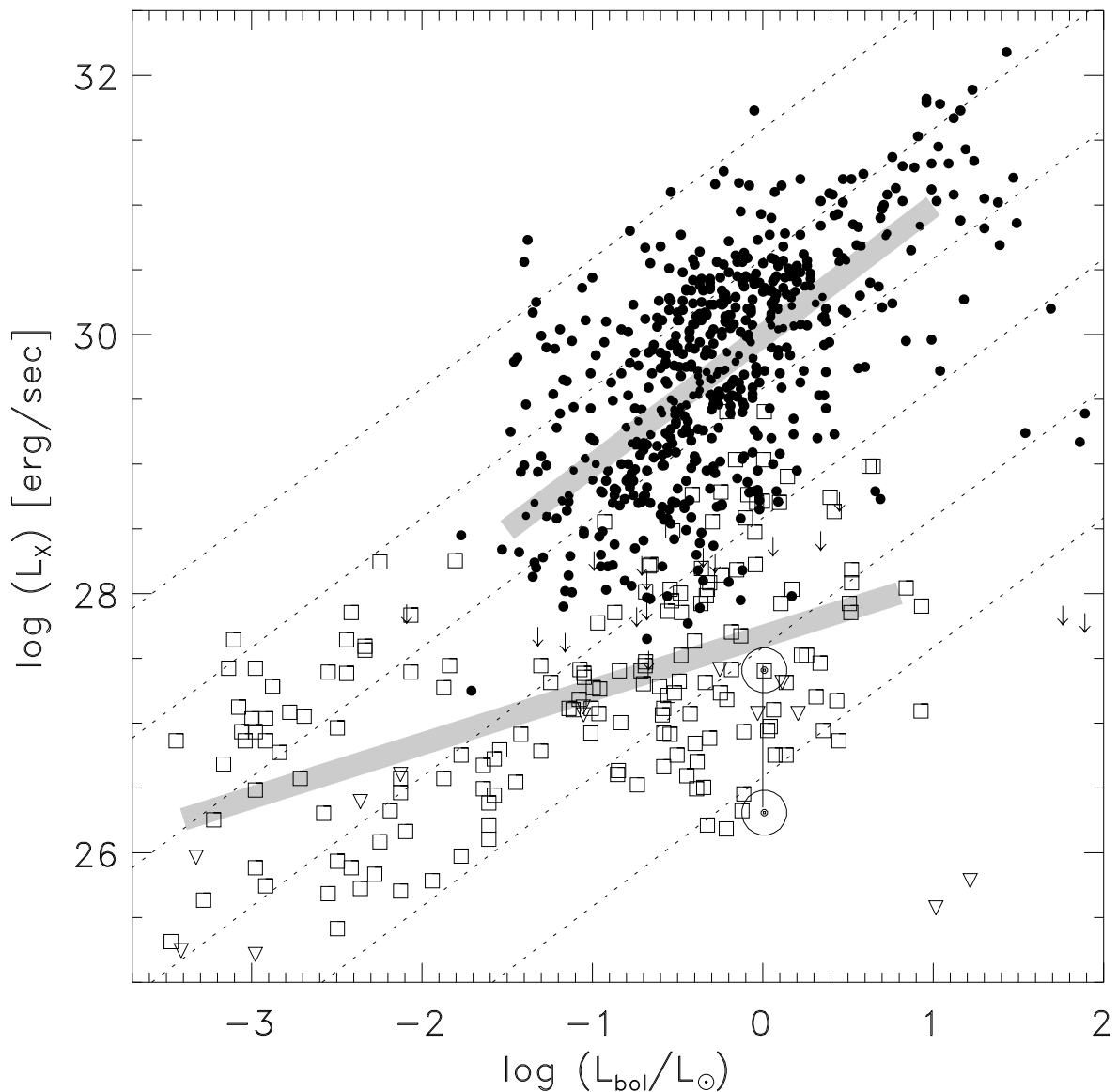
Fig. 6.— X-ray luminosity versus bolometric luminosity for the stars in the COUP optical sample (solid dots, arrows for upper limits) and for the NEXXUS sample of nearby field stars (open squares, triangles for upper limits). The dotted lines mark \log(L_X/L_{\text{bol}}) ratios of -2 , -3 , -4 , -5 , -6 , and -7 . The thick grey lines show the linear regression fits with the EM algorithm computed with ASURV for these two samples.
