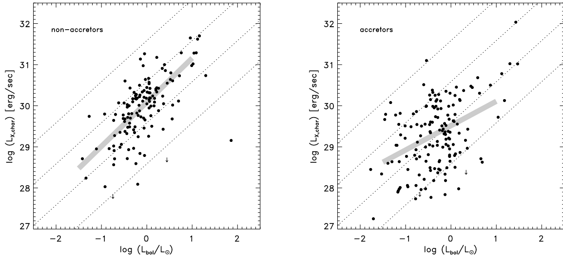
Fig. 17.— Characteristic X-ray luminosity versus bolometric luminosity for the stars in the optical sample with the 8542 \text{ \AA} Ca II line in absorption (left, non-accretors) and in emission (right, accretors). The dotted lines mark \log(L_X/L_{\text{bol}}) ratios of -2 , -3 , -4 , and -5 . The thick grey lines shows linear regression fits for L_{\text{bol}} \leq 10 L_{\odot} stars with the EM algorithm computed with ASURV.
