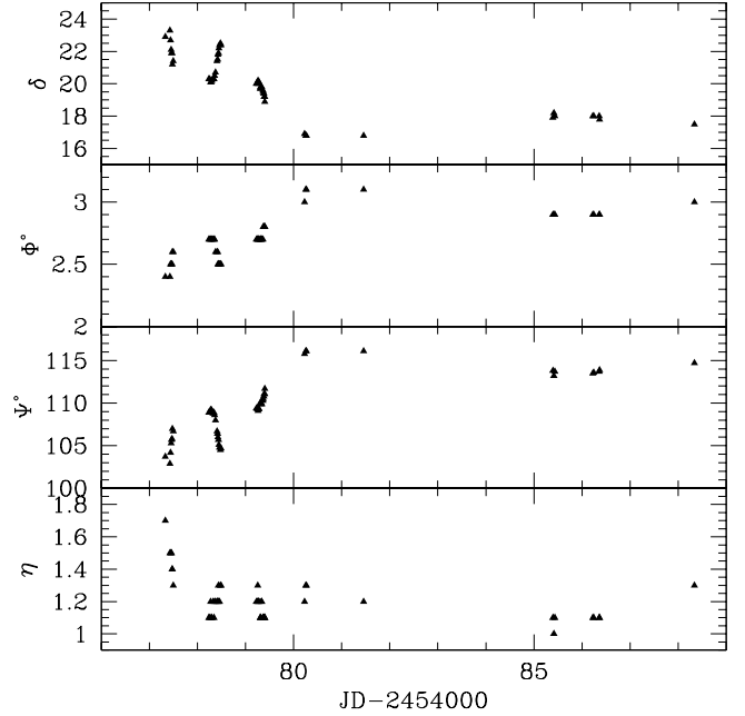
FIG. 8.—Derived values of Doppler factor, \delta , angle between the jet axis and line of sight, \Phi , viewing angle of the shock, \Psi , and compression factor of the shocked plasma, \eta .
