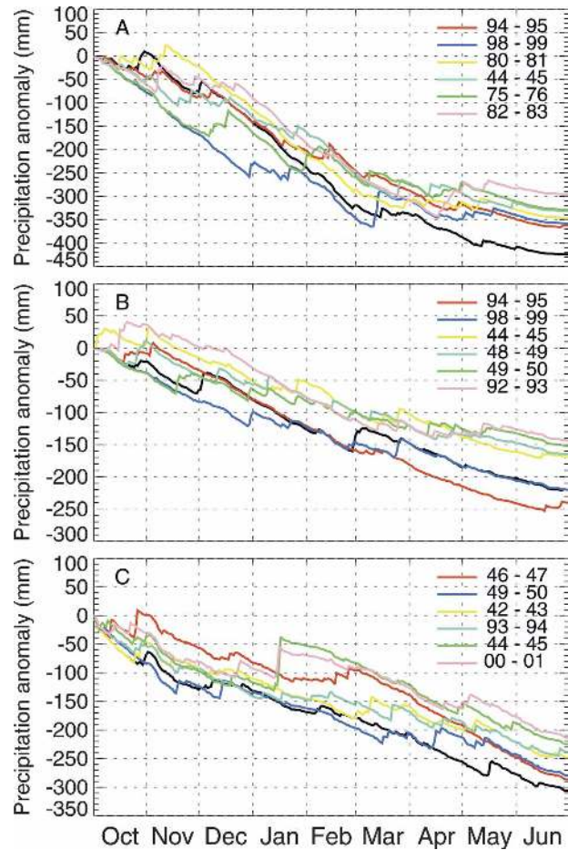
FIG. 4. Daily accumulated precipitation anomaly compared to the 1961–90 normal for the stations at (a) Reliquias, (b) Granada, and (c) Barcelona. Black line depicts the precipitation anomaly recorded during the October 2004–June 2005 period. The colored lines display the six greater droughts ever recorded in each station (1941–2005 period) during the corresponding October (year n - 1 ) to June (year n ) hydrological year.
