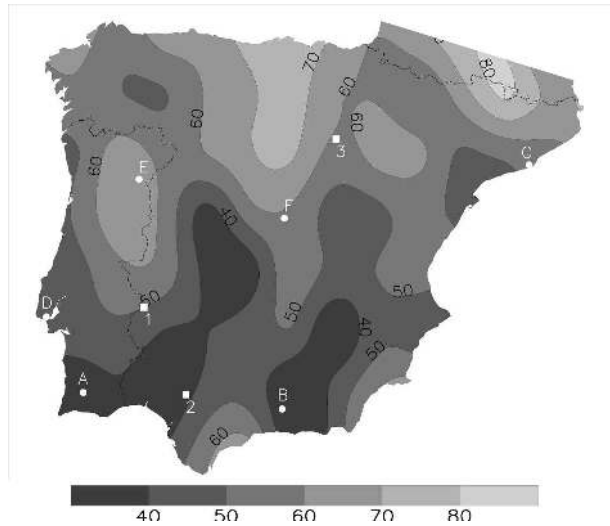
FIG. 1. October 2004–June 2005 accumulated precipitation percentage of the normal 1961–90 period for the Iberian Peninsula, using the monthly GPCP precipitation dataset: (a) the Reliquias station, (b) Granada, (c) Barcelona, (d) Lisbon, (e) Pocinho, and (f) Madrid.
