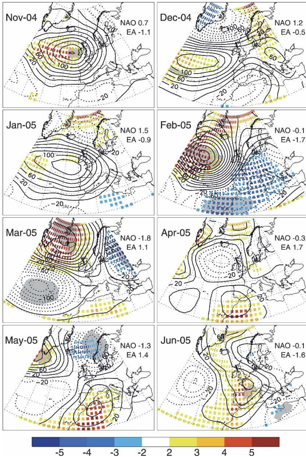
FIG. 7. Monthly anomalies of 500-hPa geopotential height (gpm; lines) and 850-hPa temperature anomaly field ( ^{\circ}\text{C} ; colored squares) between November 2004 and June 2005. The gray shading highlights those regions where the 500-hPa geopotential height anomalies are significantly different from the climatology at the 5% level. All data from ECMWF (climatology derived between 1961 and 1990). The corresponding NAO and EA monthly indexes (CPC) are displayed in the top-right corner of each panel.
