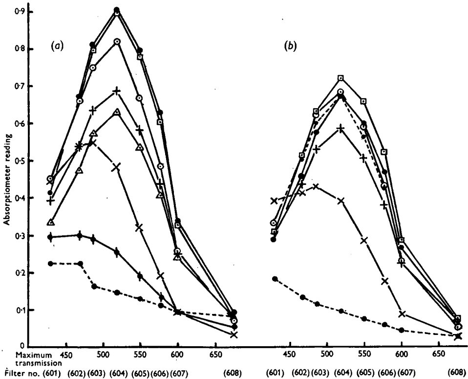
Fig. 8. Light absorption curves of pigments formed by enzymic oxidation of (a) catechol and (b) homocatechol in the presence of nitrogenous bases. Ordinates, absorptometer readings; abscissae, wave lengths of maximum transmission of the filters used, the serial number of each filter (Ilford spectrum series) being given in the appropriate position under the wave-length scale. The bases used were ●—●, proline; □—□, hydroxyproline; ○—○, hydroxyproline ethyl ester; +—+, pyrrolidine; ×—×, glycine; Δ—Δ, dimethylamine; †—†, methylamine. The broken line at the foot of each set of curves indicates the readings in a control in which no base had been present. The measurements were made at a dilution corresponding to 0.0002 M in terms of the amount of o -diphenol used, and in a 1 cm. cell. The upper broken line in (b) indicates the readings given by a 0.0002 M solution of the synthetic quinone I.
