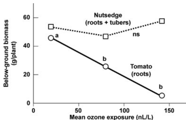
Figure 2. Differential effects of O_3 exposure on biomass allocation below-ground in a sexually reproducing species, tomato, and a vegetatively reproducing species, nutsedge (after Shrestha and Grantz 2005). Values within each line associated with different letters differ at P \leq 0.05 .
