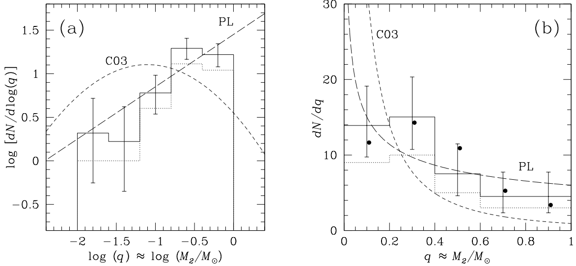
Fig. 14.— Mass ratio distribution for the 30 \leq 0.5 Gyr-old binaries in our AD 30 sample (see § 9.1) in terms of \log(dN/d \log q) (a) and dN/dq (b) . The dotted histogram traces the observed data, while the solid histogram delineates the incompleteness-corrected data. Further incompleteness due to bias against near-equal binary systems exists in the highest mass ratio bin, but has not been taken into account in the present incompleteness correction. The long-dashed line is a power-law (PL) fit to the data, dN/d \log q \propto q^{\beta+1} , with an index of \beta = -0.39 \pm 0.36 ( 1\sigma limit). The short-dashed line represents the log-normal MF of field objects from Chabrier (2003, C03) in units of M_\odot , normalized to the incompleteness-corrected data. We note that because the primary masses for stars in our sample are \approx 1 M_\odot , then q = M_2/M_1 \approx M_2/M_\odot . The log-normal field MF peaks at \mu = 0.08 M_\odot and has a width of \sigma = 0.69 (in logarithmic mass units). The Salpeter index in these units is \alpha = -2.35 . The solid points in panel (b) are the incompleteness-corrected data from Duquennoy & Mayor (1991), normalized to our data. The Duquennoy & Mayor (1991) data have been offset slightly to the right from ours for clarity.
