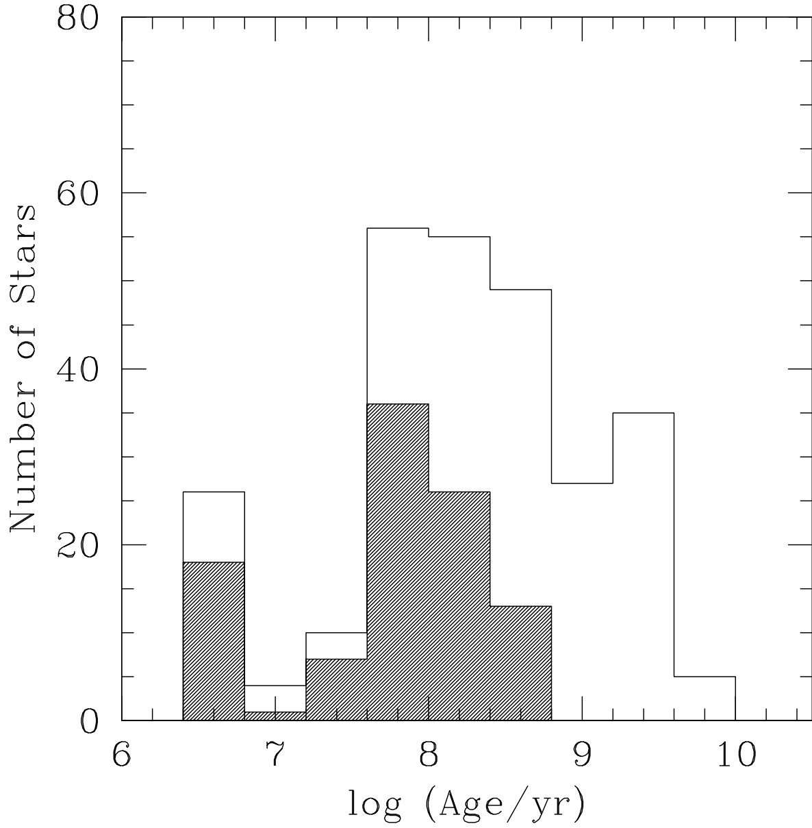
Fig. 2.— Age distributions of the complete survey sample (non-shaded histogram) and of the deep sub-sample (shaded histogram).
