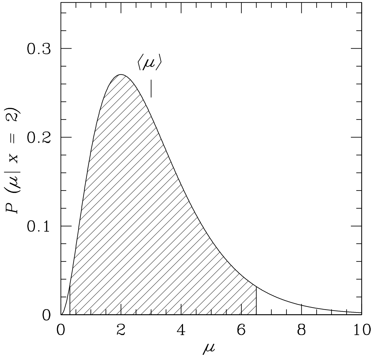
Fig. 12.— Probability density distribution P(\mu|x = 2) for the expected substellar companion detection rate in our survey per 100 stars, given x = 2 detections. The curve is a Gamma distribution (Eqn. 5), with a peak at \mu = \mu_{\text{ML}} = 2 , but a mean value of \langle \mu \rangle = x + 1 = 3 . The minimal 2\sigma (95.4%) confidence interval on \langle \mu \rangle , 0.3 < \langle \mu \rangle < 6.5 is indicated by the shaded region under the curve.
