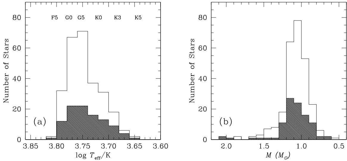
Fig. 1.— Distribution of the sample stars as a function of effective temperature (a) and mass (b). The non-shaded histograms refer to the entire sample of 266 stars, whereas the shaded histograms refer to the deep and young sub-sample of 100 stars. All stars fall in the F5–K5 range of spectral types and the majority are between 0.7 M_{\odot} and 1.3 M_{\odot} .
