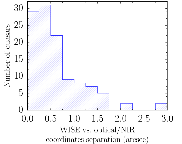
Figure 14. Separation in arcsec between the WISE and optical/near-infrared coordinates of the known z > 5.6 quasars with at least a 3\sigma detection in one of the WISE bands. The four quasars with a separation greater than 2'' are P135+16, P187-02, P242-12, and P197+25.
