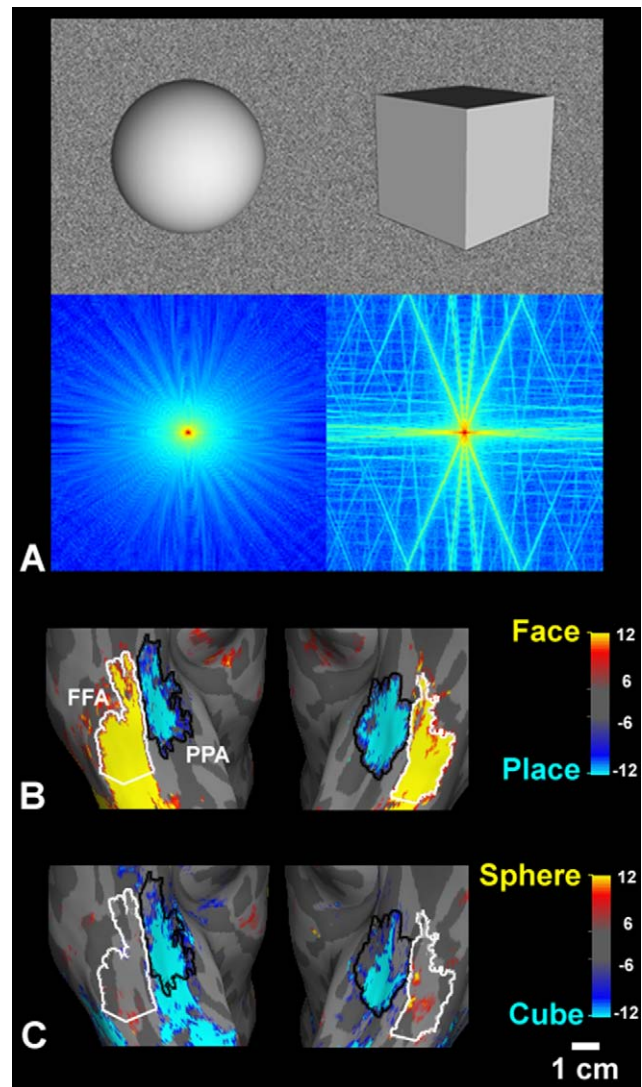
Figure 1. The higher-order cortical area PPA responds differentially to cubes versus spheres. (A) Sphere and cube stimuli and their FFTs. The top row shows sample images of the “smooth” sphere and the “smooth” cube. The bottom row shows the averaged 2-D FFT of the four sphere (left) and the four cube (right) images. The four images were distinguished only by changes in the location of the illuminant (see Materials and Methods). The red/blue color map represents the FFT magnitude (magnitude = red > yellow > cyan > blue) in Fourier space; the center of this space indicates the DC component of the FFT. The spectral distribution included a complex pattern of high SF components in the cube, but not in the sphere. Here and in the other FFT maps, the SF units are in cycles per pixel. (B) As a control, we produced an fMRI map based on a conventional, blocked-design comparison of naturalistic face versus place images, in five human subjects (using independent localizer scans). The group-averaged activity map is displayed on a ventral view of the averaged inflated cortical surface; the left hemisphere is shown on the right, with anterior towards the top. Faces and places produced relatively higher activity in FFA and PPA, respectively. (C) Relative activation to the cube versus the sphere is based on the averaged data, from the same five subjects shown in (B). The cube activated PPA robustly and selectively, with a topography similar to that produced by place-based activation. The color scale bars in the cortical maps here and in the other figures indicate the p -values, in a logarithmic format (i.e., -\log_{10}[p] ). doi:10.1371/journal.pbio.1000608.g001
