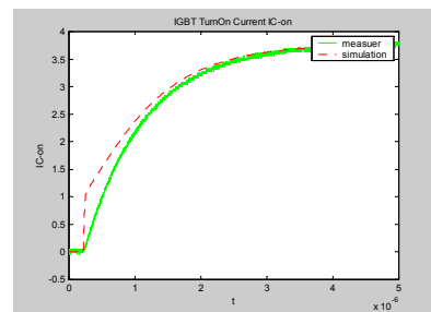
Fig. 7 The IGBT turn-on drain current I_D waveform
