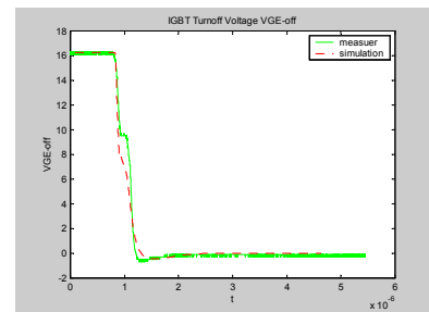
Fig. 8 The IGBT turn-off V_{GS} waveform
