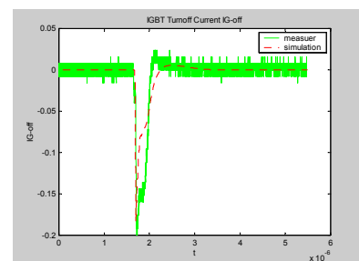
Fig. 9 The IGBT turn-off I_g waveform
