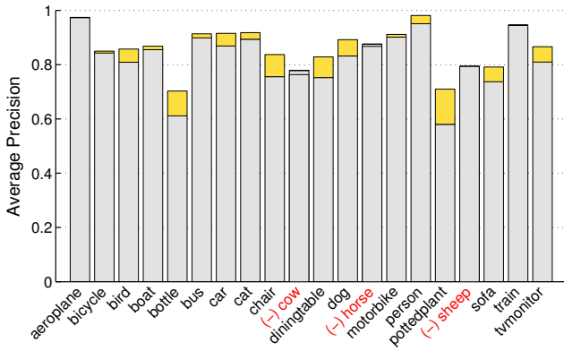
Fig. 16: AP increase of super-classifier. Gold indicates the increase in performance on object classes where the super-classifier beats all other methods, averaged across the two folds. The three classes for which performance drops slightly have been highlighted in red.
