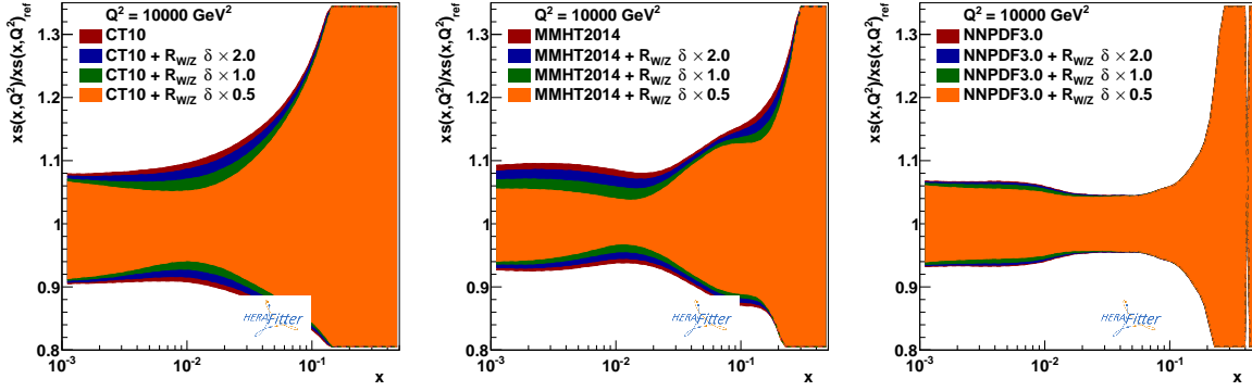
Fig. 7: Relative uncertainty of the strange-quark distribution as a function of x for Q^2 = 10^4 \text{ GeV}^2 estimated based on CT10nnlo (left), MMHT14 (middle) and NNPDF3.0 (right) PDF sets, respectively. The outer uncertainty band corresponds to the original PDF uncertainty. The embedded bands represent results of the PDF profiling using R_{W/Z} pseudo-data at 13 TeV corresponding to (from outermost to innermost band) conservative, aggressive model of the data uncertainties.
