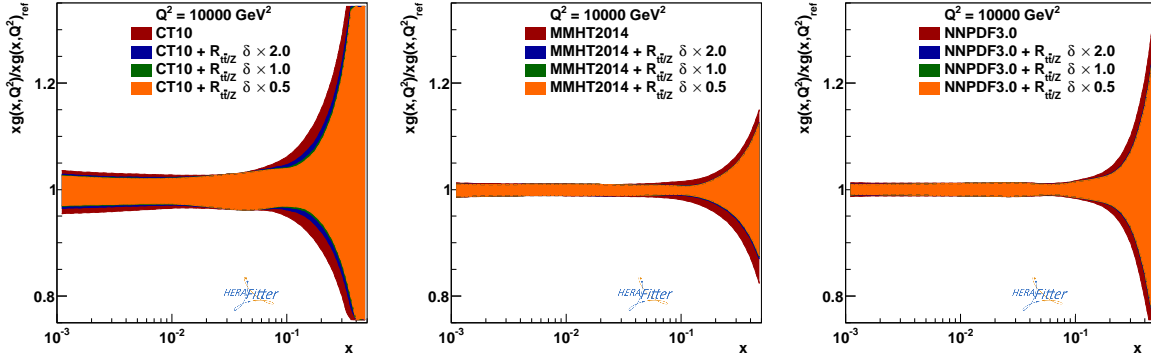
Fig. 8: Same as Fig. 7 this time for the gluon PDF, using the measurement of the t\bar{t}/Z ratio as input to the profiling.
