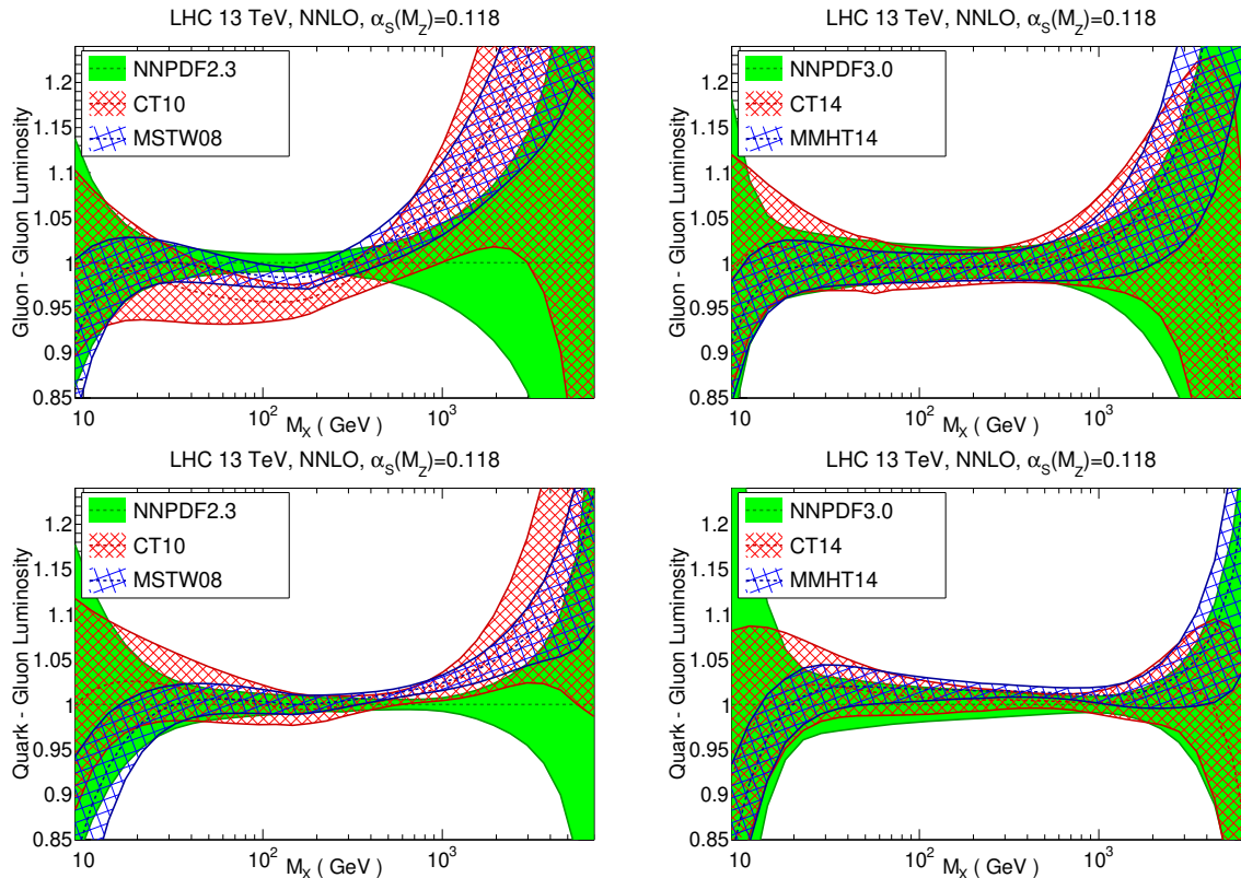
Fig. 3: Same as Fig. 2 now for the gluon-gluon (upper plots) and quark-gluon (lower plots) PDF luminosities
