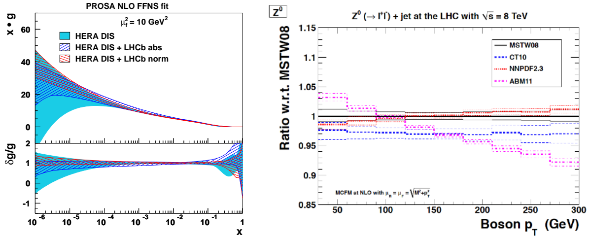
Fig. 6: Left plot: gluon distribution (top) and its relative uncertainty (bottom), shown as a function of x at the factorization scale of 10 \text{ GeV}^2 , comparing the results of the NLO QCD analysis [34] of HERA-I DIS data only (filled band) and that including either absolute or normalized cross sections of heavy-flavor production at LHCb (dashed bands). Right plot: the transverse momentum distribution of Z bosons at the LHC 8 TeV computed at NLO using various sets of PDFs, shown as ratio to the MSTW08 prediction, from Ref. [38]
