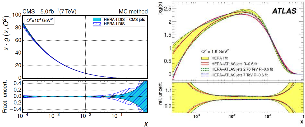
Fig. 4: Left plot: impact of the CMS 2011 inclusive jet data on the gluon PDF, from Ref. [48]. Right plot: impact of the ATLAS measurement on the ratio of inclusive jet cross-sections between 7 TeV and 2.76 TeV on the gluon PDF, from Ref. [24].
