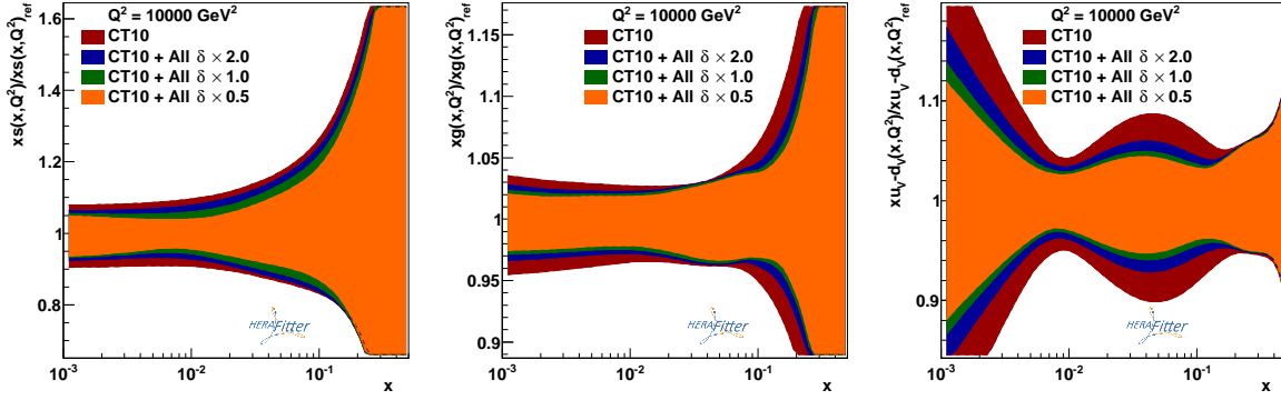
Fig. 11: Relative uncertainty of the strange-quark (left), gluon (center) and u_v - d_v (right) distributions as a function of x for Q^2 = 10^4 GeV 2 estimated based on CT10nnlo PDF set. The outer uncertainty band corresponds to the original PDF uncertainty. The embedded bands represent results of the PDF profiling using the complete set of observables considered in this exercise: R_{W/Z} , R_{t\bar{t}/Z} , A_\ell and y_Z pseudo-data at 13 TeV. The various bands correspond to (from outermost to innermost band) conservative, baseline, aggressive model of the data uncertainties.
