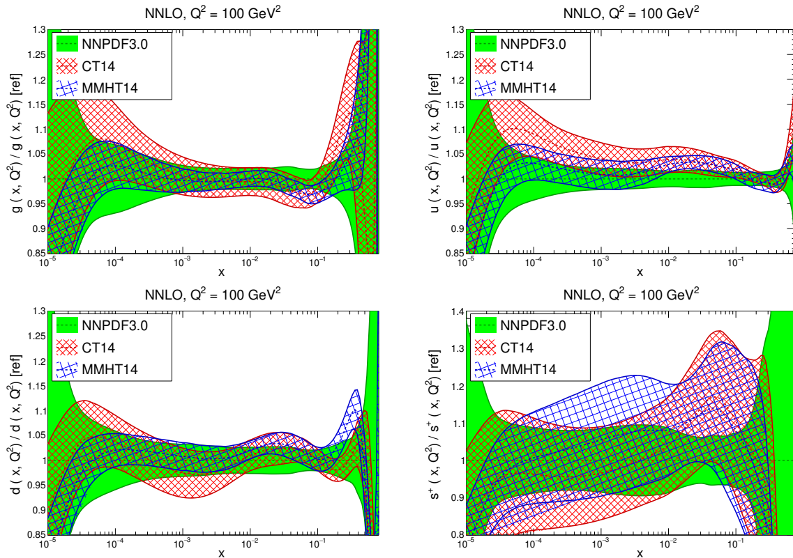
Fig. 1: Comparison of PDFs at Q^2 = 10^2 \text{ GeV}^2 between the NNPDF3.0, CT14 and MMHT14 sets, all of them at NNLO, with \alpha_S(m_Z^2) = 0.118 . From top to bottom, and from left to right, we show the gluon, the up quark, the down quark, and the total strangeness PDFs. Results are shown normalized to the central value of NNPDF3.0.
