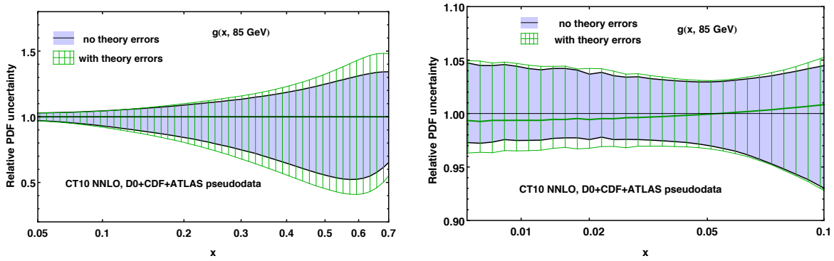
Fig. 13: Gluon PDF uncertainties at 90% C.L. for the fits with and without theoretical errors. Left plot: large- x region. Right plot: intermediate- x region.
