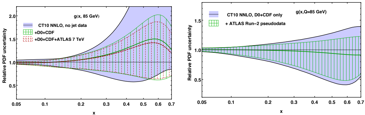
Fig. 12: Left plot: Gluon PDF uncertainties at 90% C.L. for the CT10-like fits without any jet data included, compared with the fits with the Run II D0 and CDF jet data, and with the Run I ATLAS jet data included. Right plot: same comparison, now for the fits including the Run 2 D0 and CDF jet data, and in addition with the ATLAS Run II simulated pseudo-data.
