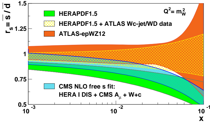
Fig. 5: The ratio of the s and d PDFs, as a function of x , compared in different analysis. We show the ATLAS results based on Z and W -boson production measurements [27] and on the associated production of W with charmed hadrons [30] as well as the CMS result [26], based on the W+c production measurement of Ref. [29]. For comparison, the HERAPDF1.5 result is also shown, where the constraints on the strange quark distribution are obtained from the neutrino-scattering experiments.
