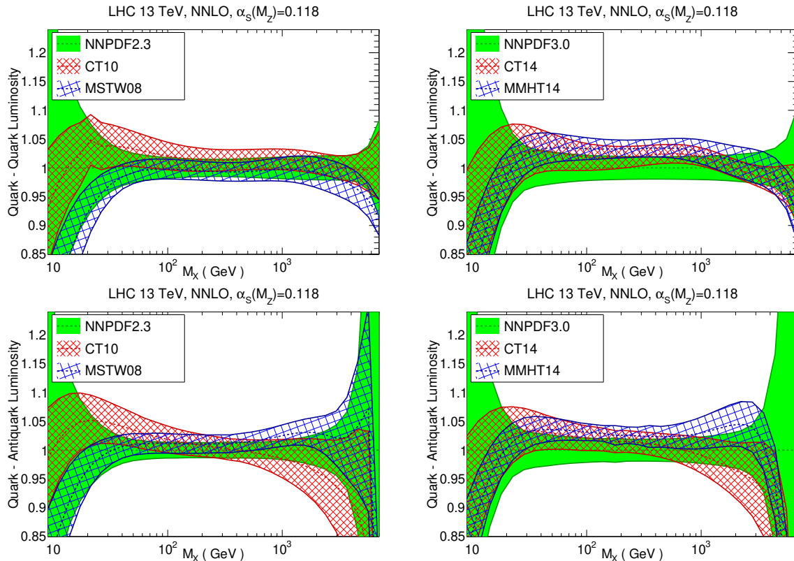
Fig. 2: Comparison of the quark-quark (upper plots) and quark-antiquark (lower plots) PDF luminosities between NNPDF2.3, MSTW08 and CT10 (left column) and the more recent NNPDF3.0, MMHT14 and CT14 (right column) PDF sets. The comparison has been performed at NNLO and \alpha_S(m_Z^2) = 0.118 for the LHC with a center of mass energy of 13 TeV, as a function of the invariant mass of the final state system M_X . Results are shown normalized to the central value of the NNPDF sets.
