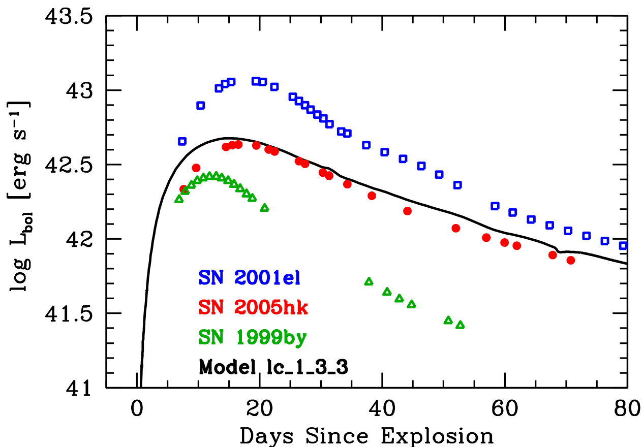
Fig. 15.— UVOIR bolometric light curve of SN 2005hk plotted with respect to the epoch of explosion. For reference, the UVOIR light curves of SN 2001el ( \Delta m_{15}(B) = 1.13 ) and SN 1999by ( \Delta m_{15}(B) = 1.90 ) are also plotted as blue squares and green triangles, respectively. For SN 2005hk, the explosion is assumed to have occurred 17 days before B maximum, whereas for SN 2001el and SN 1999by this number is taken to be 18.1 and 11.0 days before B maximum, respectively. The data for SN 2005hk are compared with the UVOIR light curve for the 3D deflagration model 1_3_3 . See text for further details.
