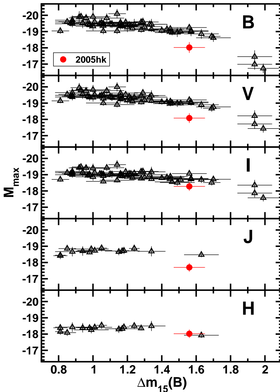
Fig. 14.— The absolute magnitudes of SNe Ia at maximum light in the BVIJH bands plotted versus the decline rate parameter \Delta m_{15}(B) . The black triangles are SNe Ia in the redshift range 0.01 < z < 0.1 whose distances were calculated from their host galaxy radial velocities in the cosmic microwave background frame assuming a Hubble constant of H_0 = 72 \text{ km s}^{-1} \text{ Mpc}^{-1} . The red circle in each panel corresponds to SN 2005hk.
