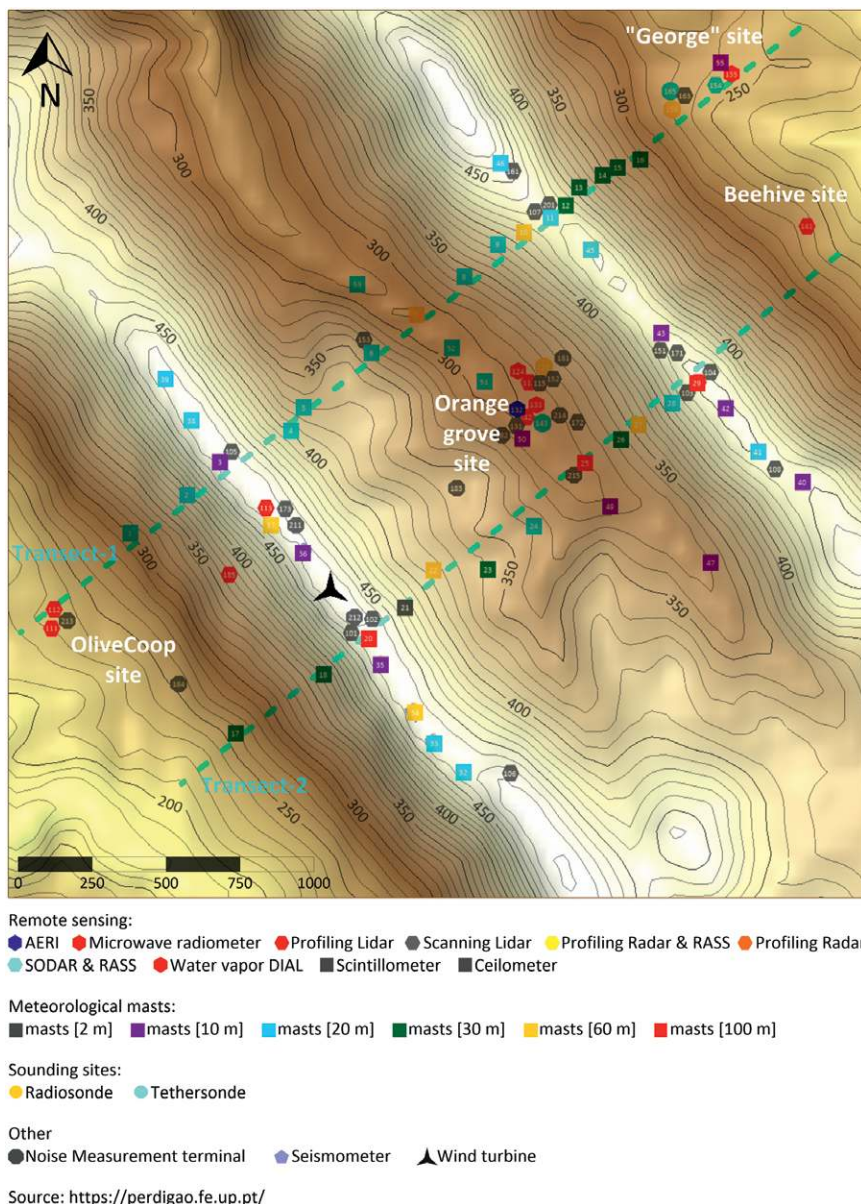
FIG. 5. Instrumentation deployed at the Perdigão campaign. Color-coded symbols indicate the type of instrumentation or tower type and the wind turbine (see legend below figure). Transects (1 and 2) and supersite locations (white lettering) are shown. A cluster of instrumentation was placed in supersites for focused process studies (also see Fernando et al. 2017).
