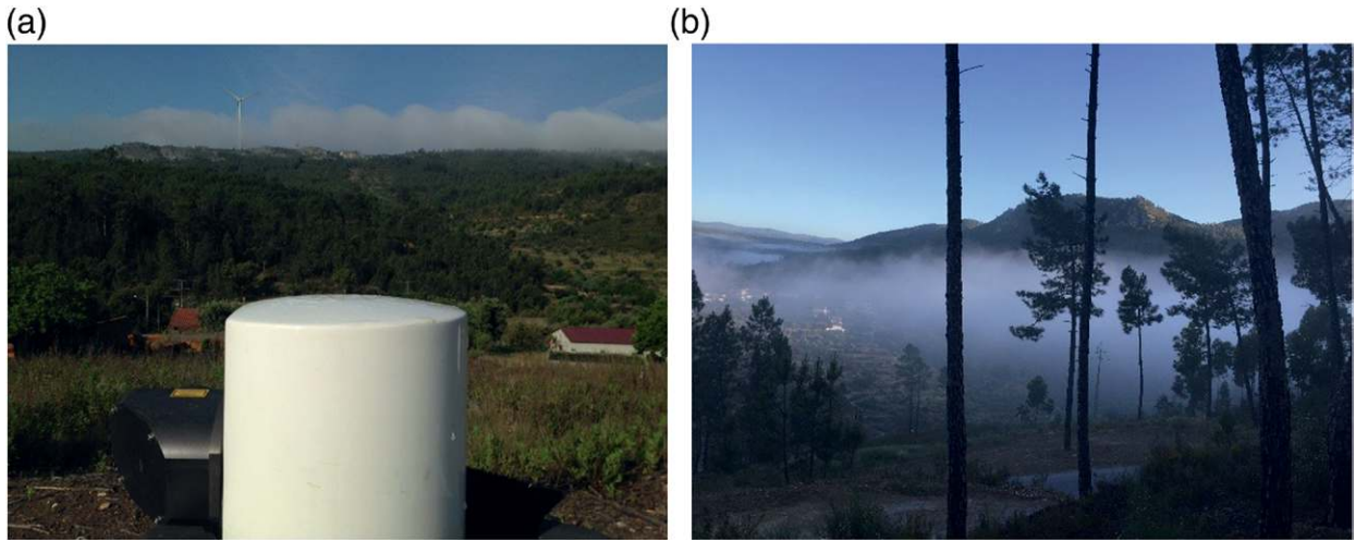
FIG. 11. (a) Low-level clouds, penetrating below the WT, viewing from the northern ridge. (b) Thinner fog layer near the valley surface, viewing from Foz do Cobre (Fig. 5).
