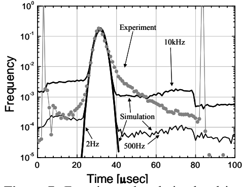
Figure 7: Experimental and simulated ion arrival-time distributions at different particle rates. The Monte Carlo simulations were made under the same electric field conditions and for the same trigger efficiency as in the experiments. The two sharp spikes in the experimental data are due to pickup from the pulsed electric field.
