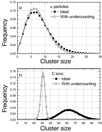
Figure 12: The effect of undercounting on simulated cluster size distributions induced by 4.25 MeV alpha (a) and 24.8 MeV carbon (b) ions. The full and open symbols represent simulated cluster size distributions without and with model-calculated undercounting, respectively. For the alpha particles (LET=107keV/ \mu m) the effect is mainly seen in the tail. For the carbon nuclei (LET= ~600keV/ \mu m) the effect is very pronounced.
