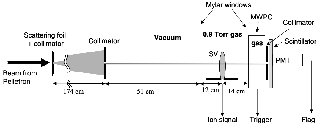
Figure 5: A schematic diagram of the beam line layout. See text.
