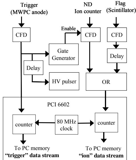
Figure 6: A flow diagram of the DAQ system. See text for details.
