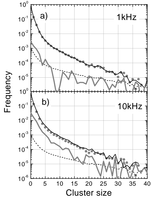
Figure 16: The effect of pile-up on the measured proton-induced cluster size distributions. The dots are the measured distributions, used as an input to a MC simulation of the pile-ups (80% trigger efficiency, pulsed mode). The thin solid line is the resulting simulated cluster size distribution in the case of a) 1kHz counting rate and b) 10kHz counting rate. The absolute difference between the two distributions is shown as a thick line. The dotted line is the expected statistical error.
