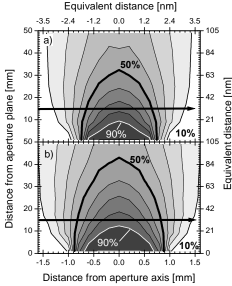
Figure 2: Monte Carlo-simulated maps of the ion extraction efficiency from the ionization volume, defining the wall-less sensitive volume. Each contour line represents a change of 10% in the ion extraction efficiency. The arrow represents the location and diameter of the collimated beam in the present experiments. The bottom and left scales are real distances in gas, while the top and right scales provide the equivalent distances in tissue. The length of the 50% contour quoted in figure 13 and in the text is measured along the SV axis, while the width is measured at the base. Figure a) corresponds to an electric field configuration: E_1 = 60\text{V/cm} , E_2 = 700\text{V/cm} and b) corresponds to E_1 = 60\text{V/cm} , E_2 = 1100\text{V/cm} . Note a factor of \sim 15 between vertical and horizontal scales
