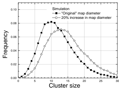
Figure 9: Simulated alpha-particle induced cluster size distributions with SV maps varying in diameter by 20%. The average cluster size differs by 40%. (Propane, 1Torr)
