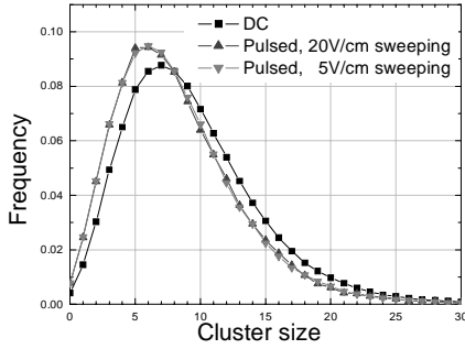
Figure 15: Cluster size distributions induced by alpha particles in DC mode, and pulsed mode with low (5V/cm) and high (20V/cm) electron sweeping fields. The pulsed field and the DC fields are 60V/cm. (Propane, 0.9 Torr)
