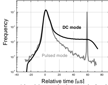
Figure 14: Measured ion arrival time distributions in pulsed (60V/cm pulse; 20V/cm electron sweeping field) and DC (60V/cm) modes. Note the large tail in DC mode, originating from the charge multiplication avalanche. (Propane, 0.9 Torr)
