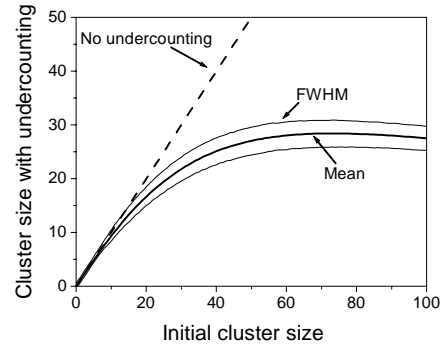
Figure 11: The simulated effect of ion undercounting, due to cluster-size dependant dead time. Shown are the mean and FWHM values of the simulated cluster size distribution as function of the initially created cluster size, taking into account the DAQ parameters. The dashed line represents the ideal case, without dead time.
