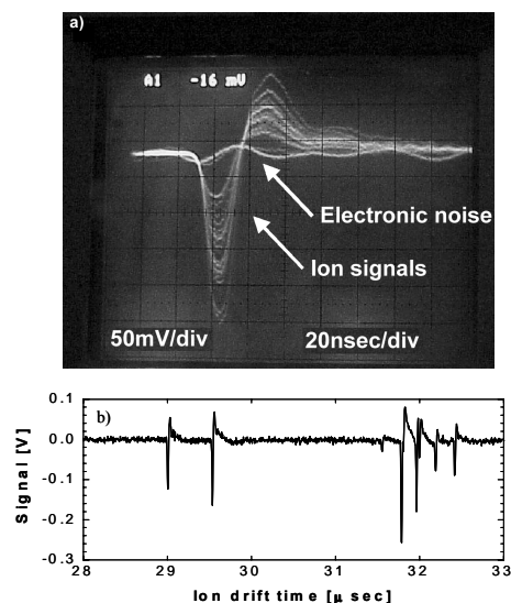
Figure 4: Examples of single ion pulses recorded from the ion counter after a fast amplifier: a) an oscilloscope photograph of single ion pulses taken off an oscilloscope. b) ion pulse train of a single event induced by an alpha particle.
