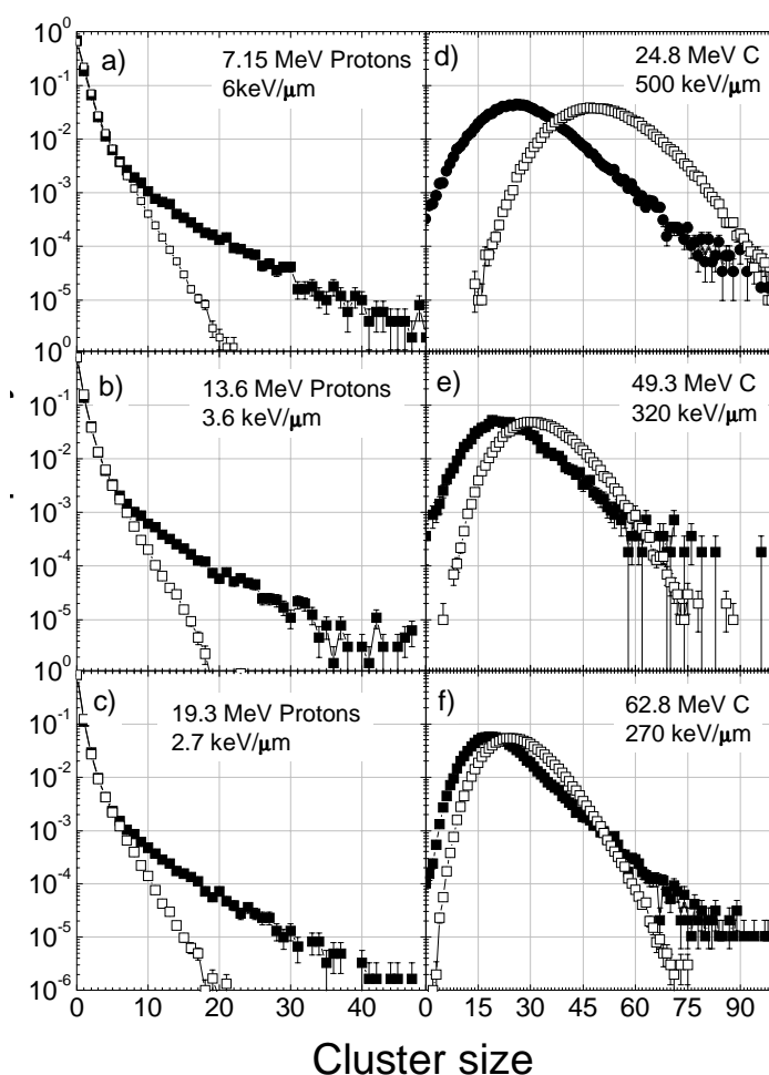
Figure 18: Experimental (full symbols) and simulated (open symbols) ionization cluster-size distributions for protons and carbon ions of different energies.
