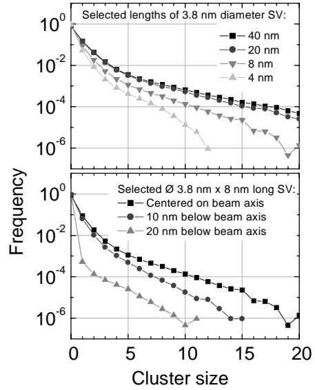
Figure 17: Experimental results of ionization cluster-size distributions, induced in selected slices along the axis of the sensitive volume shown in figure 2b. These distributions were derived from data presented elsewhere [13], selecting various ion arrival time windows, and are shown here to demonstrate the technique.
