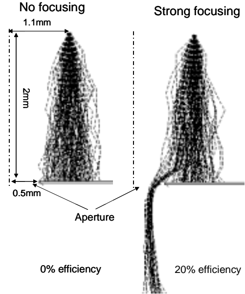
Figure 3: Simulated single ion trajectories with and without focusing for ions deposited two mm above the aperture and one mm (two aperture radii) aside from the aperture axis (denoted by the dash-dot line).
