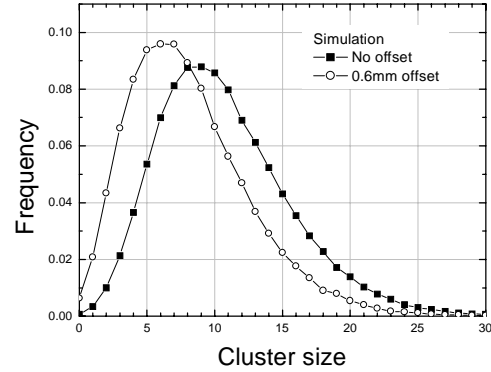
Figure 8: Simulated alpha-particle induced cluster size distributions with the beam either centered on the sensitive volume or displaced by 0.6mm. (Propane 1 Torr)
