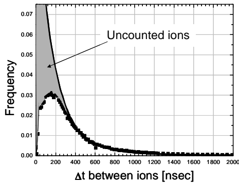
Figure 10: Measured and simulated distributions of the time difference between consecutive ions in a 40-ion cluster. The solid line is the distribution expected from simulations. About 45% of the ions are missing from the experimental one.
