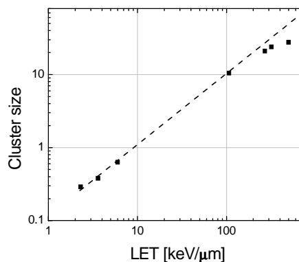
Figure 19: Dependence of the measured average cluster size in 0.9 Torr of propane, with different projectiles, on the LET (in water). The dashed line is given to guide the eye. The deviation from linearity at large LET values is due to ion-pulse undercounting as described in section 3.1.2.
