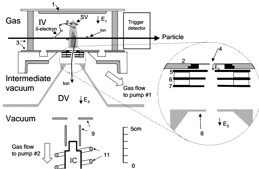
Figure 1: A detailed diagram of the ion counting nanodosimeter construction. In the ionization volume (IV), the anode (1), cathode (2) and field shaping electrodes (3) determine the extraction field E_1 . Ions created within the sensitive volume (SV), are extracted via the aperture (4) into the intermediate vacuum region; they are focused under the field E_2 , via the electrodes A_1 (5), A_2 (6), A_3 (7) and A_4 (8) into the detection volume (DV). They are then accelerated and focused, by the electrodes (9) into the ion counter (IC). A helical coil (11) protects the ion counter from discharges. Note that the SV and \delta -electron are schematic representations and not to scale.
