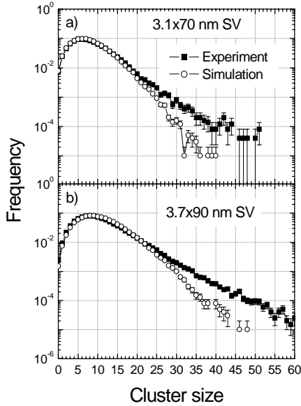
Figure 13: Experimental (full symbols) and model simulated (empty symbols) cluster size distributions induced by 4.25 MeV alpha particles in the two respective (a, b) sensitive volumes depicted in figure 2. (Propane, 0.9 Torr)
