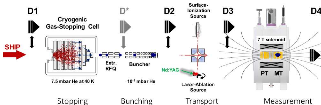
Fig. 1. Schematic view of the SHIPTRAP setup after relocation and implementation of the cryogenic gas stopping cell to stop the evaporation residues after their in-flight separation at SHIP. Further steps include ion guiding, bunching, transport, preparation and finally the high-precision PTMS. D1 to D4 indicate detector positions. The detector position D* was temporarily used. For further explanations see text.
