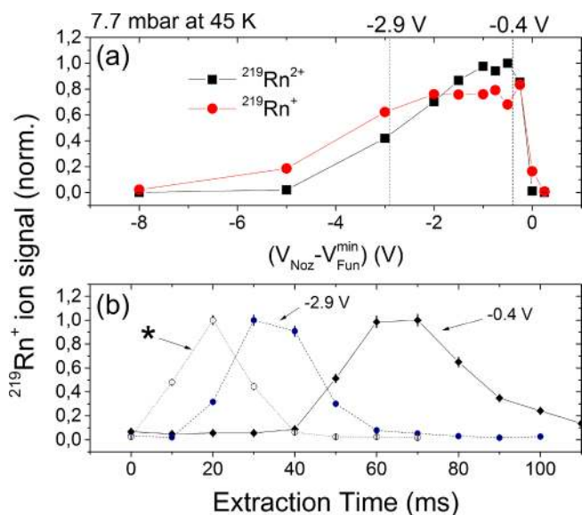
Fig. 2. Signal of the extracted ions from a ^{223}\text{Ra} recoil-ion source as a function of the voltage difference between the extraction nozzle and closest funnel electrode (a) and the extraction time (b) at a gas pressure of 7.7 mbar with an operating temperature of 45 K measured at D3. The source was placed 20 cm in front of the funnel with a DC gradient of 1.6 V/cm. The extraction time curves were measured at a voltage difference between the extraction nozzle and closest funnel electrode of -0.4\text{ V} and -2.9\text{ V} , respectively. * corresponds to -2.9\text{ V} with a higher funnel DC gradient of 3.5 V/cm along the funnel. To obtain the extraction time in (b) a pulsed source voltage in combination with a delay-pulsed extraction RFQ was used.
