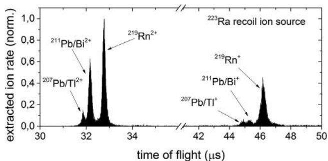
Fig. 3. Time-of-flight spectrum of extracted ions from a ^{223}\text{Ra} recoil-ion source located inside the cell (placed 20 cm in front of the extraction nozzle) measured at D3. The gas pressure was 7.3 mbar at an operating temperature of 40 K. The buncher was operated at 100\text{ V}_{\text{pp}} with a buncher accumulation time of 40 ms. The starting time corresponds to the ejection pulse from the buncher.
