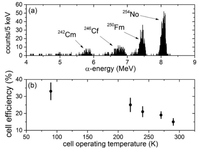
Fig. 4. (a) \alpha -decay spectrum of extracted 254 No ions measured at D*. The data was summed over 21 successive measurements with a total measurement time of about 6600 s. (b) Cell efficiency \epsilon_{\text{cell}} as a function of the cell operating temperature.
