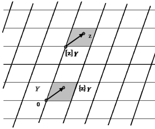
FIG. 1. Definition of [z]_Y and \{z\}_Y .
