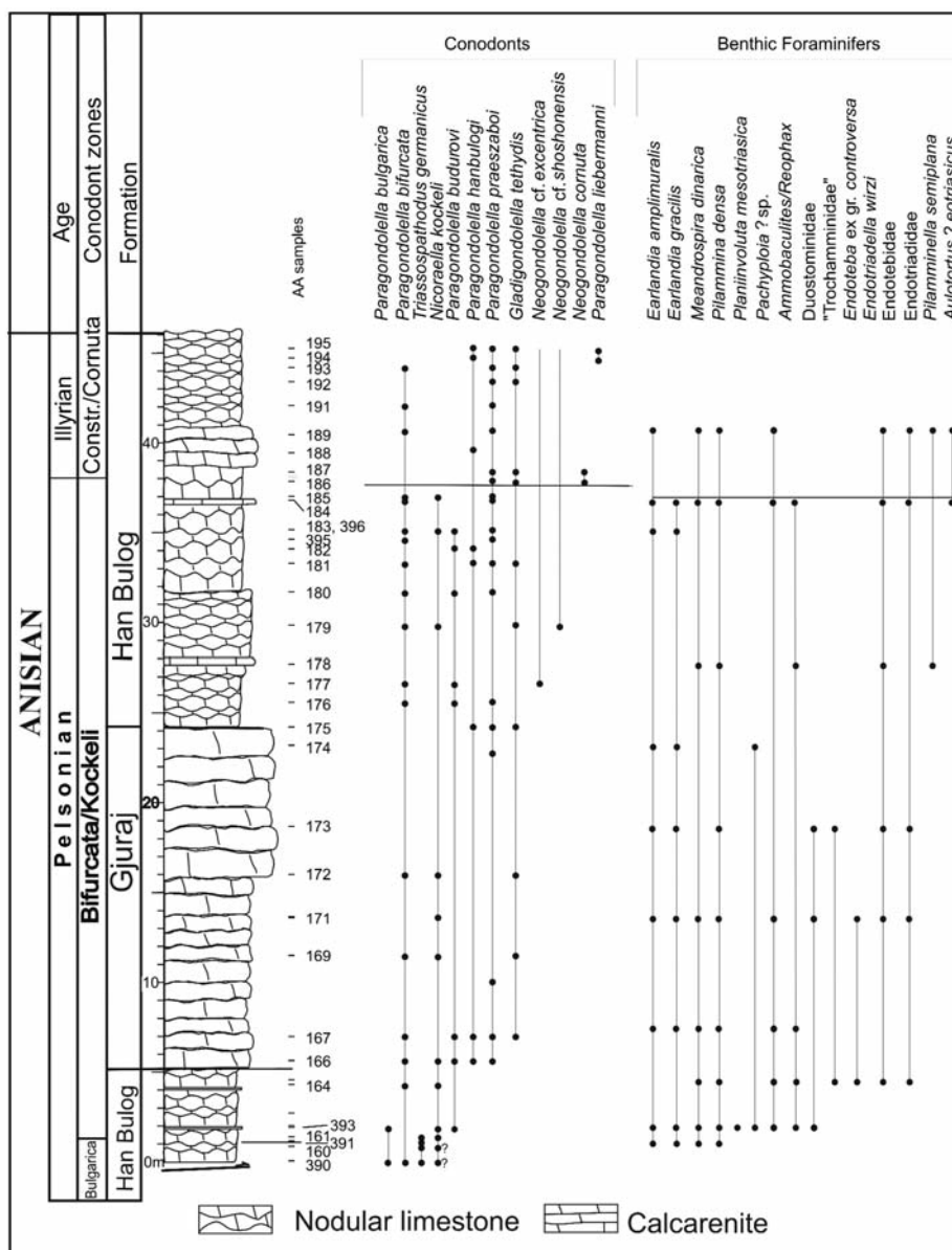
Text-fig. 8. The section of Nderlysj [from Muttoni et al. 1998, simplified]. The Pelsonian /Illyrian boundary is slightly different according to conodonts and foraminifers. To save space the label AA (Albanian Alps) is omitted
