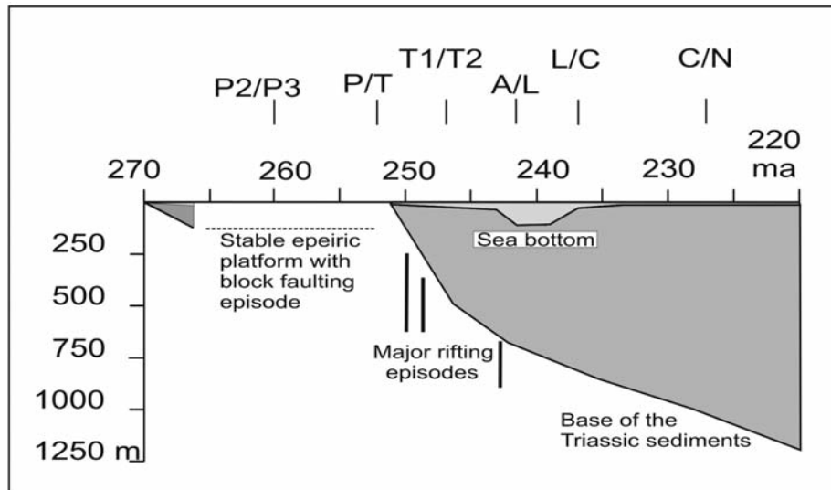
Text-fig. 10. Tentative subsidence curve for the Triassic of Albanian Alps. Thickness of sediments not decompacted. The most important subsidence occurred during the Early Triassic, when thick conglomerate bodies were deposited. Numeric ages according to Mundil et al. (2010) and Ogg et al. (2014)
