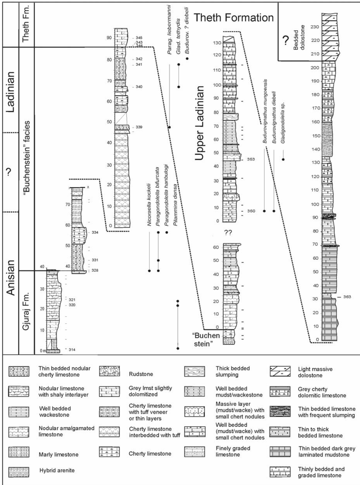
Text-fig. 9. The composite sections measured around the village of Theth. The Gjuraj, "Buchenstein", and lower part of the Theth formations were measured in the deep gully to the south of the village, from 970 m to 1170 m a.s.l. After a grassy flat, starting at about 1250 m a.s.l, along the gully above and to the north of the road, the remaining part of the Theth Fm. was measured. To save space the label AA (Albanian Alps) is omitted
