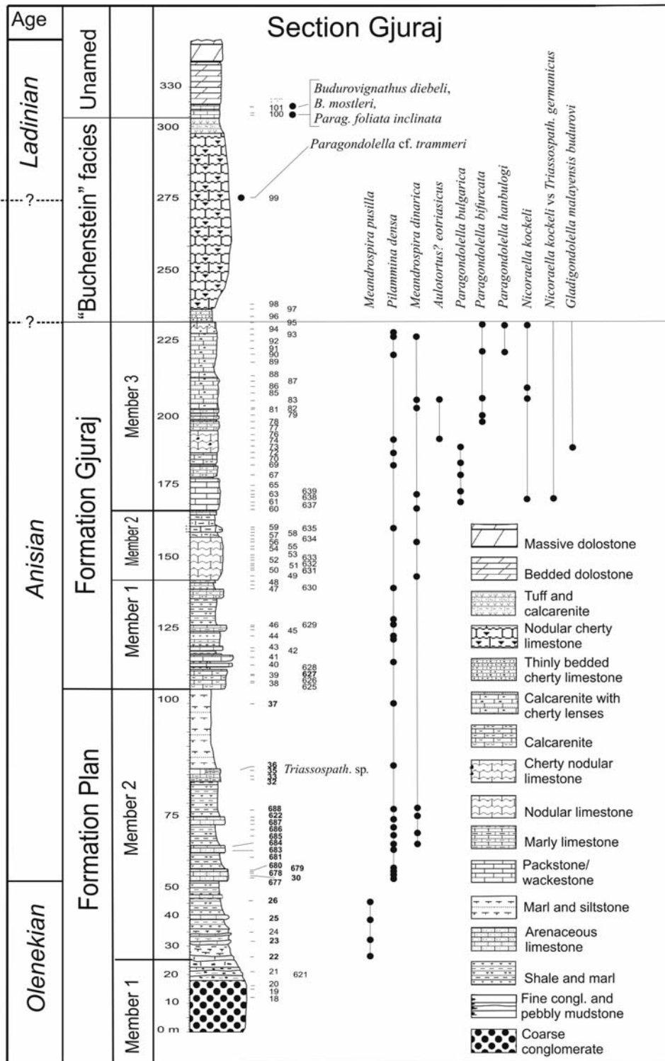
Text-fig. 6. The Gjuraž section, with the formations of Plan, Gjuraž, the Buchenstein facies and an unnamed unit are better exposed. The ranges of conodonts and of the most significant foraminifers are reported. To save space the label AA (Albanian Alps) is omitted
