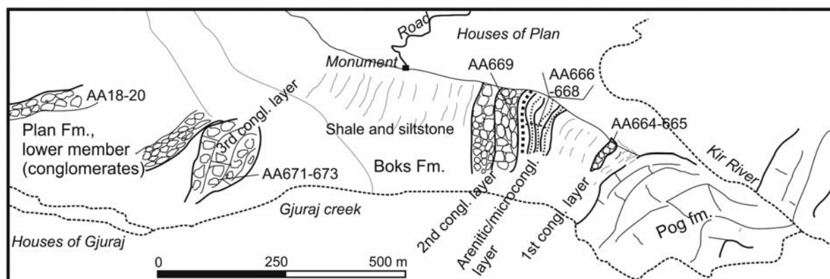
Text-fig. 5. The ridge where the conglomerates of the Boks and Plan formations are better exposed. Position of samples is indicated. The drawing is based on the oblique view from Google Earth
