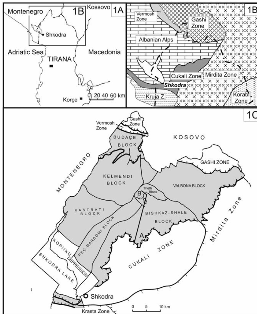
Text-fig. 1. Index map of the study area (1A and B), with structural map of the Albanian Alps (1C) [from Xhomo et al. (2008), simplified]
