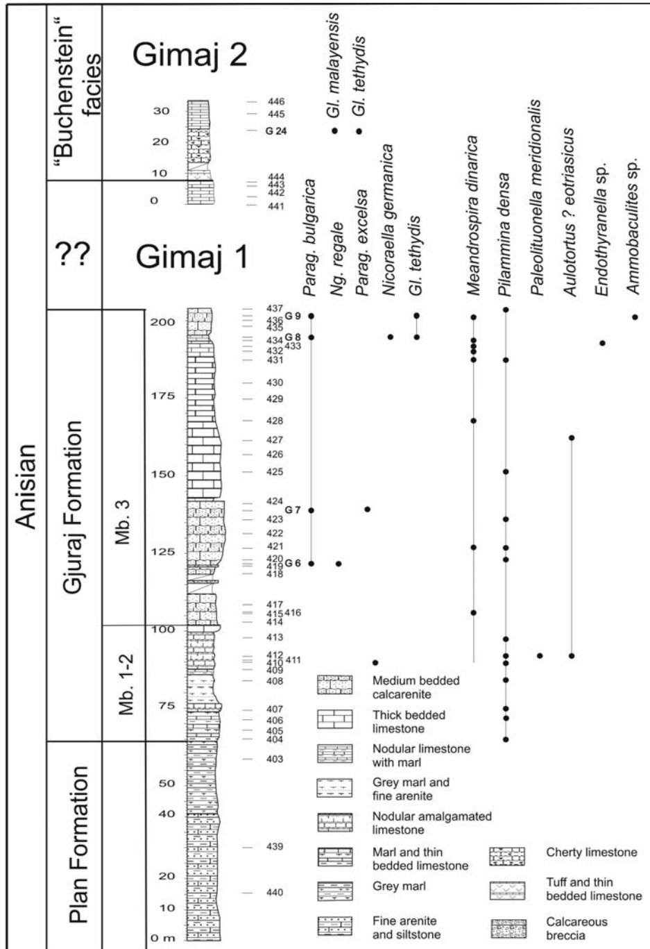
Text-fig. 7. The composite section of Gimaj. Base of the log Gimaj 1: 940 m a.s.l.; N 42°18'57", E 19°45'07". Base of log Gimaj 2: 870 m a.s.l.; N42°19'07", E 19°45'16". To save space the label AA (Albanian Alps) is omitted. Sample G are conodont samples
