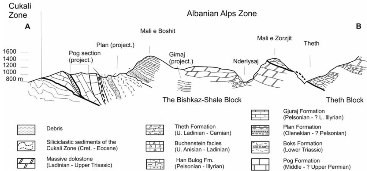
Text-fig. 3. Geological cross-section across the study area; for location see Text-fig. 2
