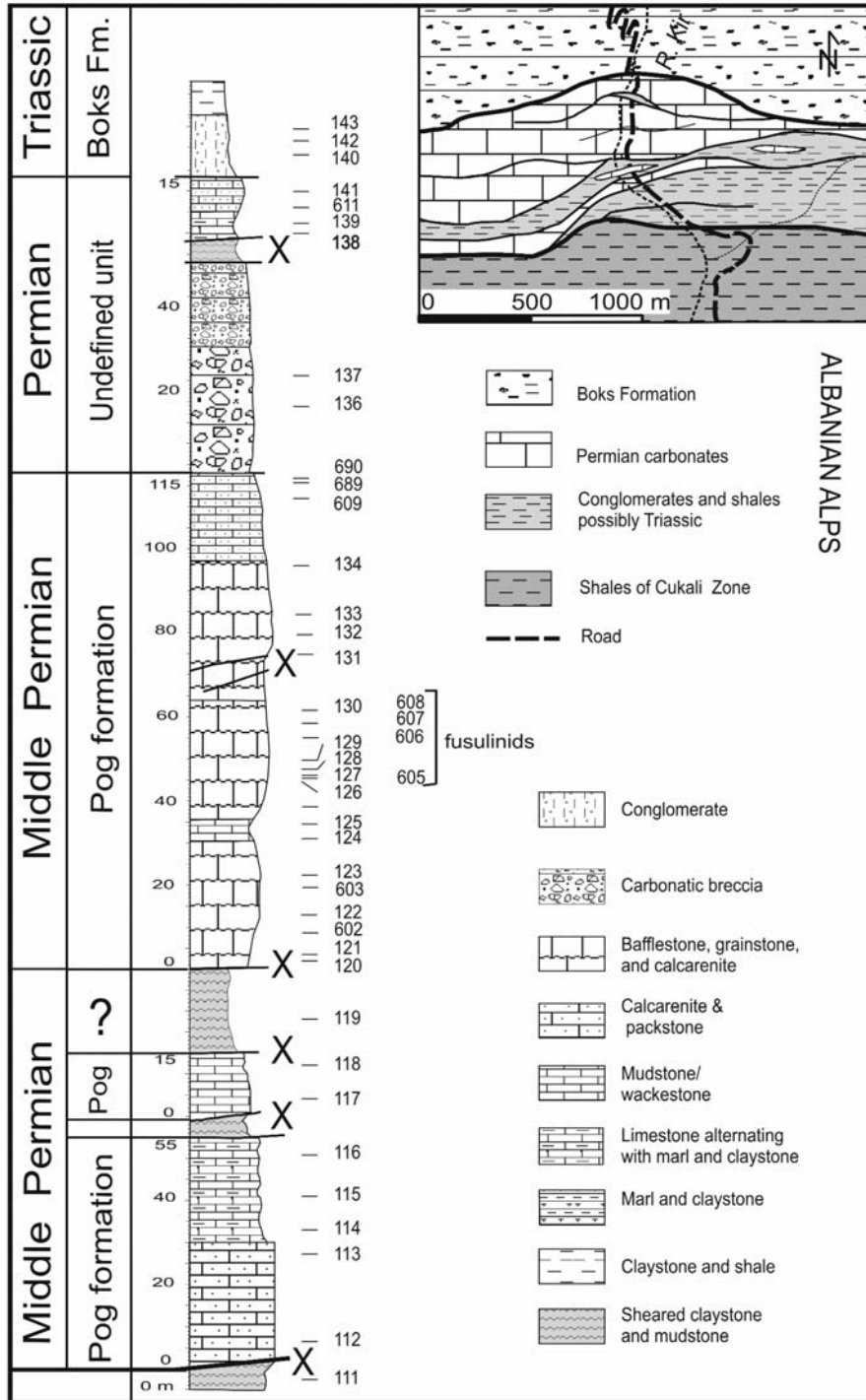
Text-fig. 4. Stratigraphic log of the Permian of Pog, measured along the road. To save space on the drawings the label AA (Albanian Alps) is omitted. Geological map of the area north of the village of Pog is inserted in upper-right corner. The road curves mentioned in the text where the first Meandrosira pusilla (Ho, 1959) have been obtained from the Boks Formation, are shown on the map
