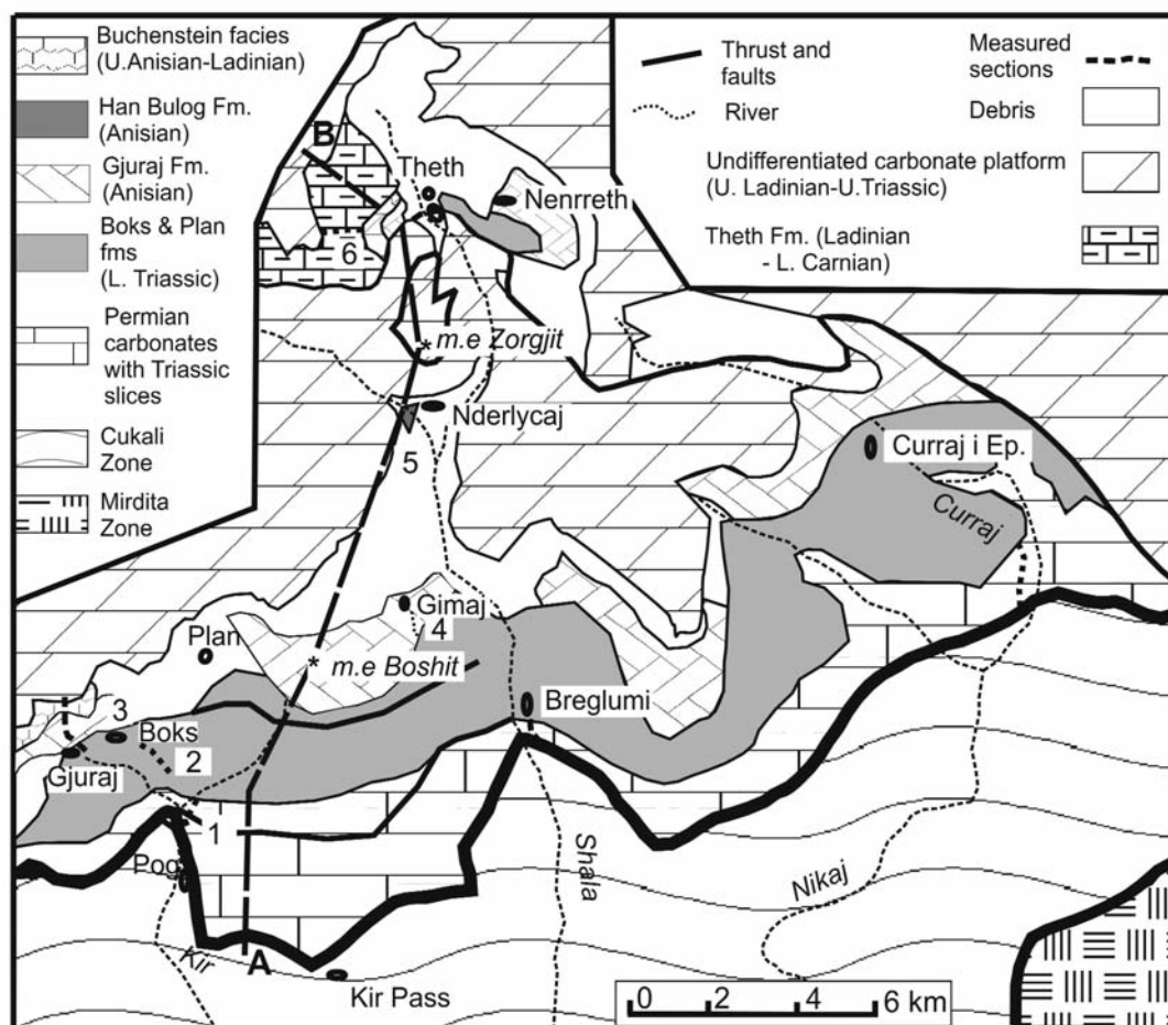
Text-fig. 2. Geological sketch-map of the study area, based on ISPGJ-IGJN (1983) geological map. Studied stratigraphic sections: 1 – Pog; 2 – Boks; 3 – Gjuraj; 4 – Gimaj; 5 – Nderlycaj; 6 – Theth. A-B – cross-section of Text-fig. 3
