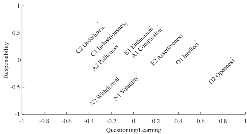
Figure 2. Plot of predictor loadings for predicted solution (PCA on SoMe subscales predicted by BFAS aspects) displayed in Table 4.
