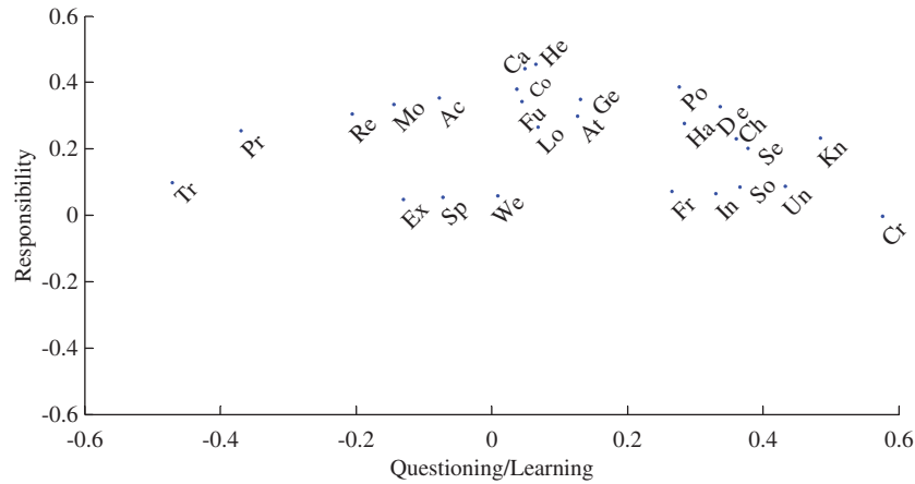
Figure 1. Plot of component loadings for predicted solution (PCA on SoMe subscales predicted by BFAS aspects) displayed in Table 3. Notes: Ac=Achievement, At=Attentiveness, Ca=Care, Ch=Challenge, Co=Community, Cr=Creativity, De=Development, Ex=Explicit Religiosity, Fr=Freedom, Fu=Fun, Ge=Generativity, Ha=Harmony, He=Health, In=Individualism, Kn=Knowledge, Lo=Love, Mo=Morality, Po=Power, Pr=Practicality, Re=Reason, Se=Self-Knowledge, So=Social Commitment, Sp=Spirituality, Tr=Tradition, Un=Unison with Nature, and We=Wellness.
