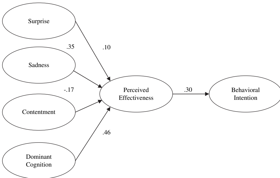
Figure 1 Structural equation model derived from the Victor Crawford data.
