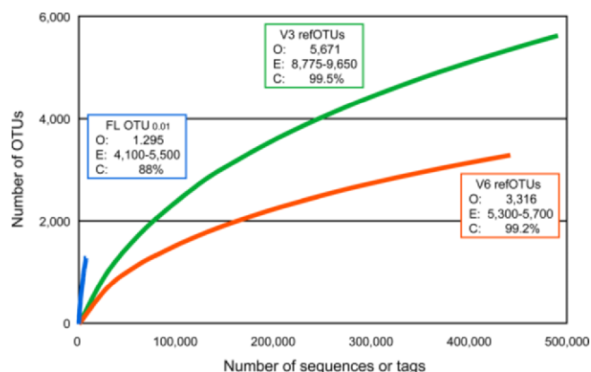
Figure 3. Rarefaction Curves
