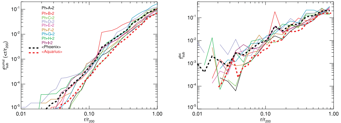
Figure 17. Left-hand panel: cumulative fractional contribution of subhaloes (resolved with more than 100 particles) to the enclosed mass, shown as a function of radius for all level 2 Phoenix clusters (thin lines). A thick dashed black curve shows the average trend, computed after stacking all nine Phoenix haloes. The corresponding result for Aquarius is shown by the thick dashed red curve. Right-hand panel: fraction of total mass contributed by substructure in different radial bins. As in the left-hand panel, only subhaloes with more than 100 particles are considered; black and red thick dashed lines correspond to the average trend computed after stacking all level 2 Phoenix and Aquarius haloes, respectively.
