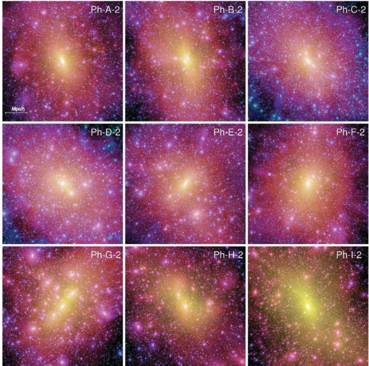
Figure 3. The same as Fig. 1, but for all level 2 Phoenix clusters at z = 0 . Boxes are all 5 h^{-1} Mpc on a side. Note that the appearance of several Phoenix clusters is suggestive of a transient evolutionary stage, characterized by the presence of undissolved substructure groupings. Ph-G-2 is a particularly good example of this irregular structure which may be traced to its recent assembly time; this cluster has acquired half its mass since z = 0.18 .
