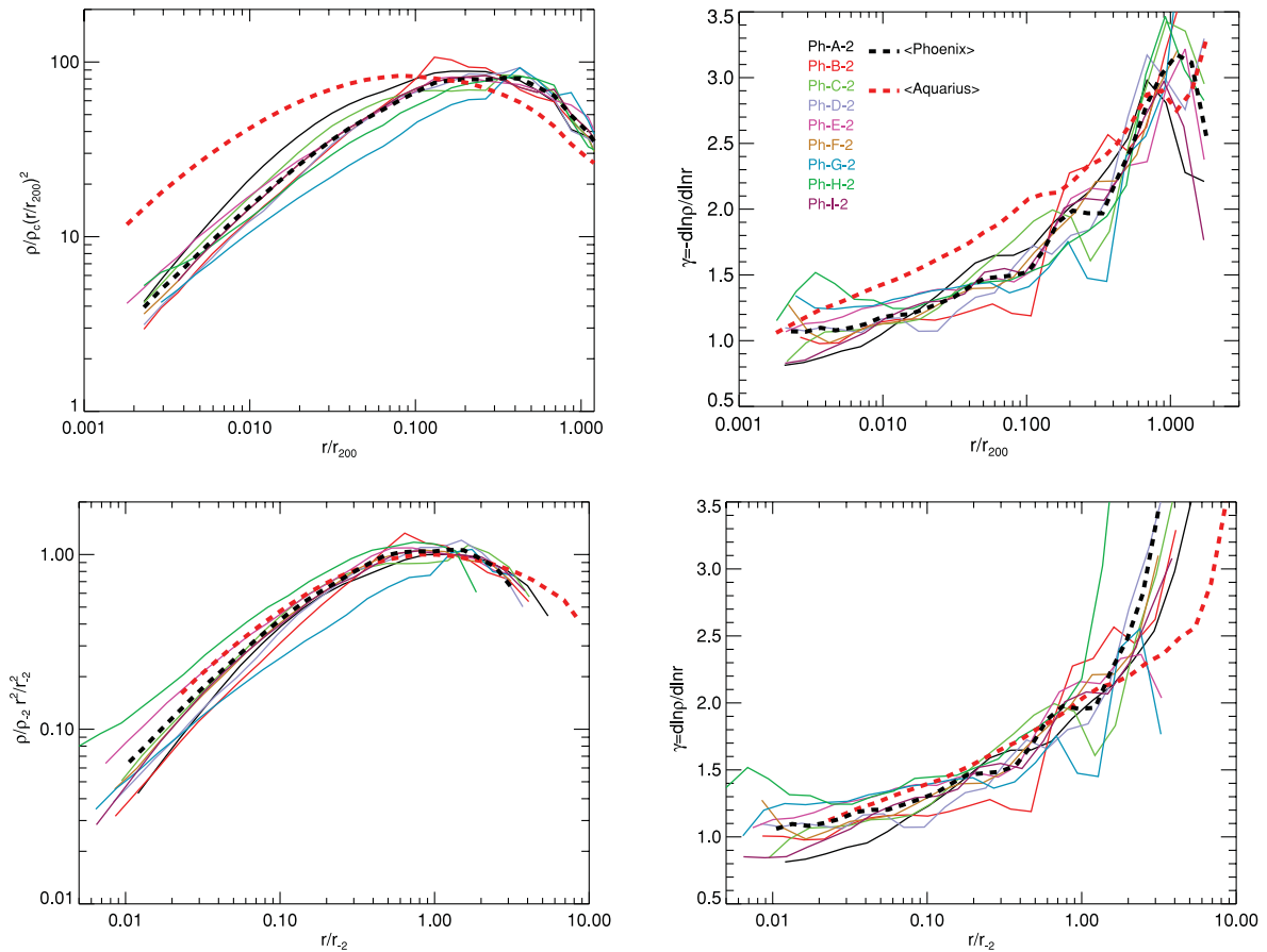
Figure 5. Spherically averaged density (left-hand panels) and logarithmic slope (right-hand panels) of all level 2 Phoenix haloes as a function of radius. Radii have been scaled to the virial radius of each halo in the top panels and to the ‘scale radius’, r_{-2} , of the best-fitting Einasto profile in the bottom panels. Profiles are plotted down to the convergence radius, r_{\text{conv}} . The thick dashed black line shows the average density profile of all Phoenix haloes, computed after stacking the nine haloes, each scaled to its own virial mass and radius. The thick red dashed line shows the result of the same stacking procedure, but applied to the Aquarius haloes.
