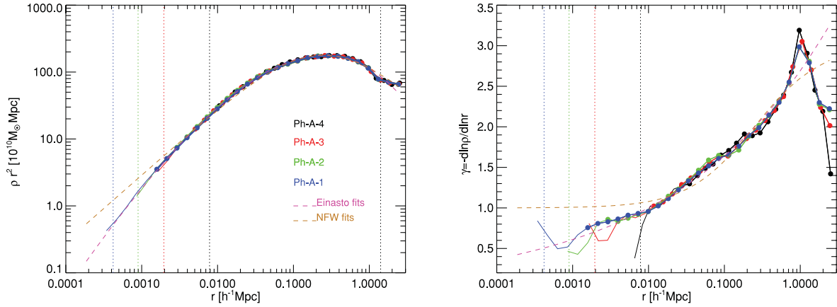
Figure 4. Left-hand panel: spherically averaged density profile of halo Ph-A at z = 0 . Different colours correspond to the four different resolution runs listed in Table 1. The panel on the left shows the density multiplied by r^2 in order to enhance the dynamic range of the plot. Each profile is shown with a thick line connecting filled circles from the ‘convergence radius’, r_{\text{conv}} , outwards (Power et al. 2003). The thin curves extend the profiles inwards down to r = 2\epsilon , where \epsilon is the Plummer-equivalent gravitational softening length. The vertical dotted lines indicate, for each run, 2.8\epsilon , the distance beyond which pairwise particle interactions are fully Newtonian. Note the excellent numerical convergence achieved for each simulation outside their r_{\text{conv}} . An NFW profile with concentration c = 5.63 (thin dashed brown line) and an Einasto profile with \alpha = 0.22 and c_E = 5.59 (thin dashed magenta line) are also shown for comparison. Right-hand panel: logarithmic slope ( \gamma = -d \ln \rho / d \ln r ) of the density profile as a function of radius. Colours and line types are the same as in the left-hand panel. Note again the excellent convergence achieved in all runs at radii outside the convergence radius, r_{\text{conv}} .
