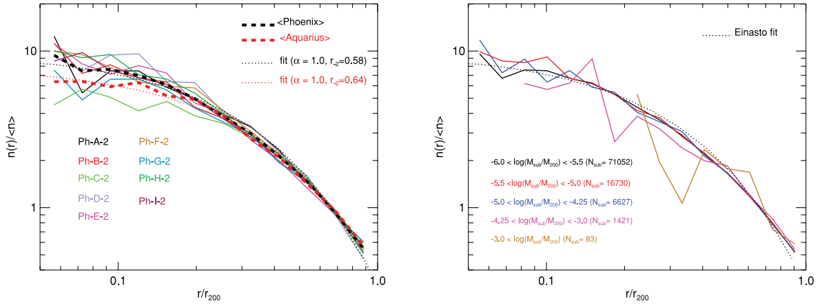
Figure 15. Subhalo number density profiles. The panel on the left shows the spatial distribution of subhaloes with more than 100 particles in each of the nine Phoenix level 2 clusters. Each profile is normalized to the mean number density of subhaloes within the virial radius. The thick dashed black curve traces the result of stacking all nine level 2 Phoenix haloes. The profile obtained after stacking all level 2 Aquarius haloes is shown by the red dashed curve. Note that subhaloes are slightly more concentrated in the case of Phoenix than of Aquarius. The panel on the right shows the density profile of subhaloes in different bins of subhalo mass, computed after stacking all nine level 2 Phoenix clusters. Note that the spatial distribution of subhaloes is approximately independent of subhalo mass.
