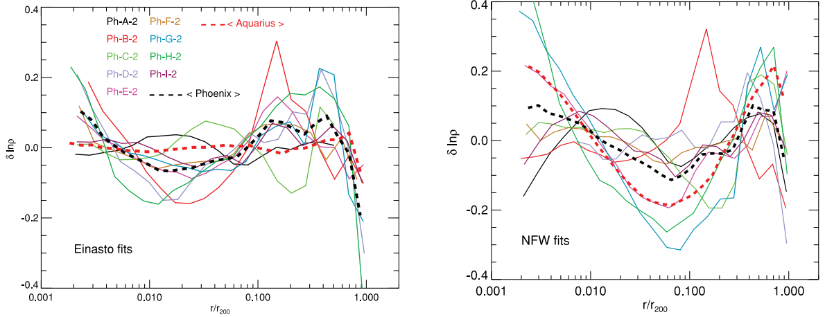
Figure 6. Residuals from the best Einasto (left-hand panel) and NFW (right-hand panel) profile fits for all level 2 Phoenix haloes. Colours and line types are as in Fig. 5. The thick black dashed curve corresponds to the composite profile obtained after stacking all nine Phoenix level 2 runs. The red thick dashed curve corresponds to the same composite profile, but for the six galaxy-sized level 2 Aquarius haloes.
