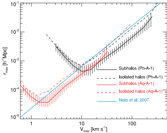
Figure 14. Peak circular velocity, V_{\max} , versus the radius at which it is reached, r_{\max} . The solid cyan curve indicates the r_{\max} – V_{\max} relation obtained for isolated haloes in the Millennium Simulation by Neto et al. (2007). Subhaloes in both Phoenix (solid black curve) and Aquarius (solid red curve) deviate systematically from this relation towards smaller r_{\max} at a given velocity. This is a result of tidal stripping, which shifts the location of the peak inwards while changing little the peak velocity. Isolated haloes identified in Aquarius and Phoenix (shown with dashed lines) are not subject to tides and are in good agreement with the Millennium Simulation results.
