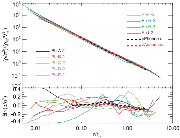
Figure 7. Spherically averaged PPSD ( \rho/\sigma^3 ) of all level 2 Phoenix haloes as a function of radius. Profiles are plotted down to the convergence radius, r_{\text{conv}} . Radii are given in units of the scale radius, r_{-2} , of the best-fitting Einasto profile for each halo. Densities are scaled to \rho_{-2} = \rho(r_{-2}) and velocity dispersions, \sigma(r) , to the characteristic velocity V_{-2} = (G\rho_{-2})^{1/2} r_{-2} . The thick dashed lines show the average PPSD of all Phoenix (black) and Aquarius (red) haloes plotted over the converged radial range common to both simulation series: 0.06 \leq (r/r_{-2}) \leq 4 , respectively. The bottom panel shows residuals from a simple r^{-1.875} power-law fit.
