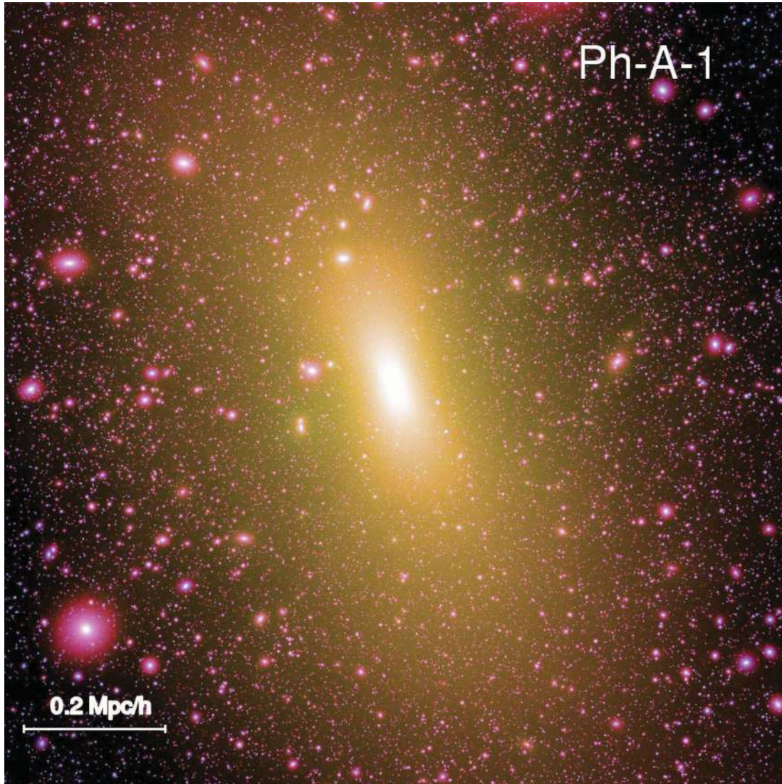
Figure 2. The inner \sim 1 h^{-1} Mpc of Ph-A-1. Colour coding is the same as in Fig. 1. This figure illustrates clearly the strong asphericity of the halo, the presence of several nested levels of substructure and the tendency of subhaloes to avoid the halo centre.
