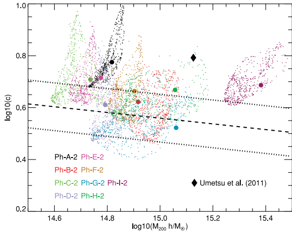
Figure 10. Cluster virial mass versus concentration estimated from fits to the projected density profiles of level 2 Phoenix haloes in the radial range R < 500 h^{-1} kpc. A total of 500 random projections are used for each halo. The large filled circles indicate the true value of the virial mass and concentration of the cluster, obtained from NFW fits to the 3D spherically averaged profile (see Appendix A and Table 2). The dashed curve flanked by dotted lines shows the fit to the mass–concentration relation derived by Neto et al. (2007). Note that projection effects lead to significant bias in the mass and concentration, which are underestimated on average by 8.5 \pm 17 and 0.4 \pm 20 per cent, respectively, where the ‘error’ is the rms of all projections for the nine clusters. The black diamond symbol indicates the M_{200-c} estimate for a stack of four strong-lensing clusters taken from Umetsu et al. (2011).
