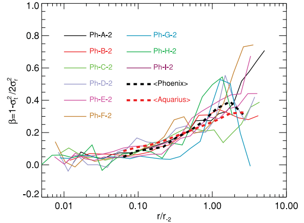
Figure 8. Velocity anisotropy profiles of all level 2 Phoenix haloes. Radii are expressed in units of the scale radius, r_{-2} , of the best-fitting Einasto profile. Profiles are plotted down to the convergence radius, r_{\text{conv}} . The thick dashed lines show the average anisotropy profile of all Phoenix (black) and Aquarius (red) haloes over the radial range where both give converged results ( 0.06 \leq (r/r_{-2}) \leq 4 ).
