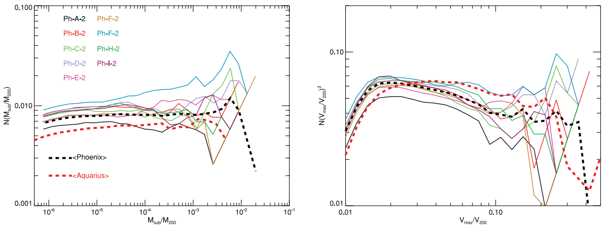
Figure 13. As the bottom panels of Fig. 12, but for all level 2 Phoenix haloes. The cumulative mass function (left-hand panel) is weighted by subhalo mass, expressed in units of the virial mass. A cumulative N \propto M^{-1} dependence, the critical case for logarithmic divergence in the total substructure mass, corresponds to a horizontal curve in these scaled units. Although the dependence is nearly flat in several Phoenix clusters it is clearly declining in others, and the average trend seems to be subcritical. Compared with Aquarius (thick dashed red curve) the average Phoenix subhalo mass function is slightly steeper. The panel on the right is analogous to the mass function, but for the subhalo peak circular velocity, weighted by V_{\max}^3 . (See the text for further discussion.)
