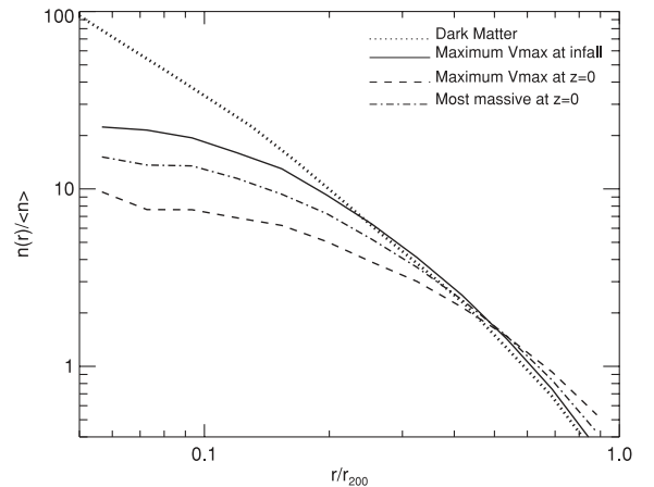
Figure 16. Stacked subhalo number density profiles as a function of r/r_{200} for the nine Phoenix haloes and for different definitions of the lower subhalo ‘mass’ limit. The solid line shows the radial profile for all subhaloes whose progenitors had a maximum circular V_{\max} exceeding 45 \text{ km s}^{-1} when they first fell into the cluster; the dot-dashed line shows a similar profile but for subhaloes with V_{\max} greater than 30 \text{ km s}^{-1} at the present day; finally, the dashed line show the profile for all subhaloes containing more than 200 bound particles. For comparison, a dotted line shows the stacked dark matter mass profile of the clusters. The profiles are normalized to integrate to the same value within r_{200} . Note that none of the subhalo profiles matches the shape of the dark matter profile within 0.25r_{200} .
