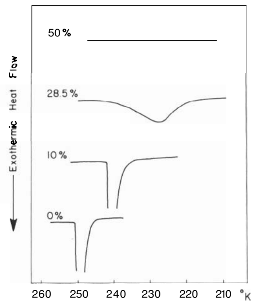
FIGURE 18. Cooling thermograms of various concentrations of bovine hemoglobin in 9M urea with AgI crystals.
