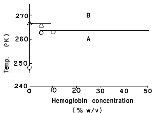
FIGURE 3. Freezing temperature of bovine hemoglobin solution in the presence (B) and absence (A) of \text{AgI} crystals.
