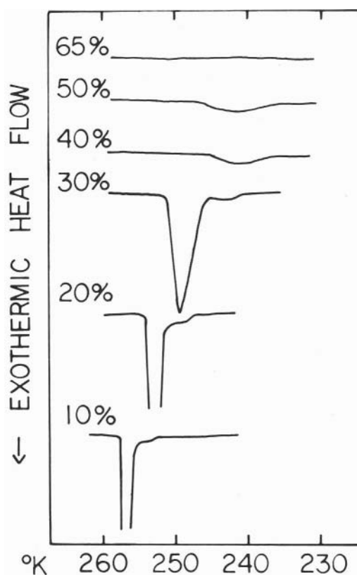
FIGURE 4. Cooling thermograms of various concentrations of PVME solutions without AgI crystals.
