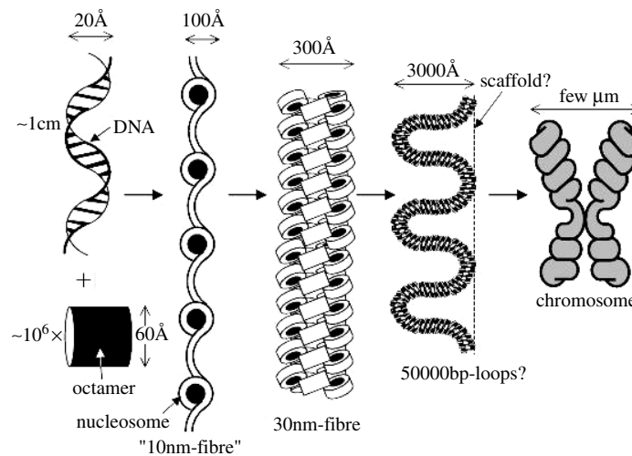
Figure 1. Steps of the DNA compaction into chromatin. The DNA molecule of length \sim 1 cm is compacted with the help of 10^6 histone octamers leading to a 10 000-fold reduction of its original length (see text for details).
