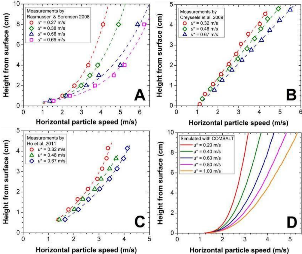
Figure 2.11. Vertical profiles of the horizontal particle speed in steady state saltation from the wind-tunnel measurements of (a) Rasmussen and Sorensen (2008), (b) Creyssels et al. (2009), and (c) Ho et al. (2011) show that the particle speed converges to a common value near the surface (see also Figure 2.12). This is reproduced by numerical saltation models (panel (d) and figure 23 in Durán et al. , 2011). All results are for particle sizes of \sim 250 \mu\text{m} .
