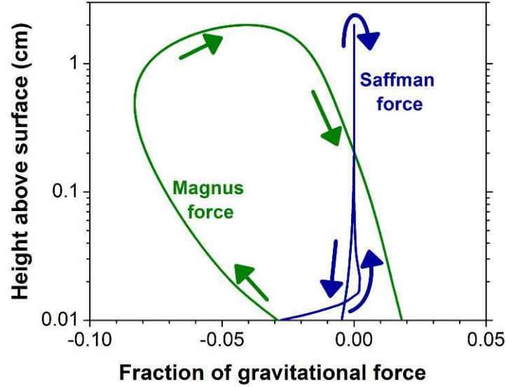
Figure 2.3. The Magnus force (green line) and the Saffman force (blue line) as a fraction of the gravitational force during the saltation trajectory of a 200\ \mu\text{m} particle launched from the surface with a speed of 1\ \text{m/s} at an angle of 40^\circ from horizontal and a rotational speed of 400\ \text{rev/s} . The arrows indicate the direction of particle motion. The particle trajectory and lift forces were calculated using Eqs. 1 – 6 in Kok and Renno (2009a), using the vertical profile of the horizontal wind speed of Eq. (2.18) with u_* = 0.20\ \text{m/s} and z_0 = D_p/30 . The asymmetries in the relative strength of both the Magnus and the Saffman force on the upward and the downward trajectories are due to changes in the velocity of the particle relative to the flow, which determines the strength and direction of these forces. The effects of turbulence were neglected.
