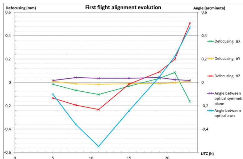
Fig.11. PILOT telescope optical alignment evolution during the first flight (ceiling altitude reached at 4h UTC).
