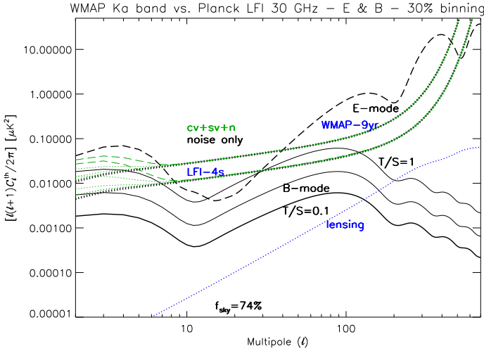
Figure 3. CMB E polarization modes (black long dashes) compatible with WMAP data and CMB B polarization modes (black solid lines) for different tensor-to-scalar ratios of primordial perturbations ( T/S = 1, 0.3, 0.1 , at increasing thickness) are compared to WMAP (Ka band, 9 years of observations) and LFI (30 GHz, 4 surveys) sensitivity to the APS (Knox 1995), assuming subtracted the noise expectation. The plots include cosmic and sampling variance plus instrumental noise (green dots for B modes, green long dashes for E modes, labeled with cv+sv+n ; black thick dots, noise only) assuming a multipole binning of 30%. Note that the cosmic and sampling (74% sky coverage) variance implies a dependence of the overall sensitivity at low multipoles on T/S (again the green lines refer to T/S = 1, 0.3, 0.1 , from top to bottom), which is relevant for parameter estimation; instrumental noise only determines capability to detect the B mode. The B mode induced by lensing (blue dots) is shown for comparison.
