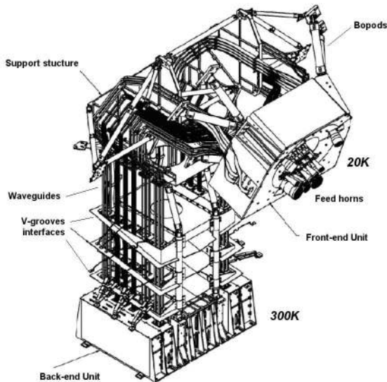
Figure 7. The LFI radiometer array assembly, with details of the front-end and back-end units. The front-end radiometers are based on wide-band low-noise amplifiers, fed by corrugated feedhorns which collect the radiation from the telescope. A set of composite waveguides transport the amplified signals from the front-end unit (at 20 K) to the back-end unit (at 300 K). The waveguides are designed to meet simultaneously radiometric, thermal, and mechanical requirements, and are thermally linked to the three V-groove thermal shields of the Planck payload module. The back-end unit, located on top of the Planck service module, contains additional amplification as well as the detectors, and is interfaced to the data acquisition electronics. The HFI is inserted into and attached to the frame of the LFI focal-plane unit.
