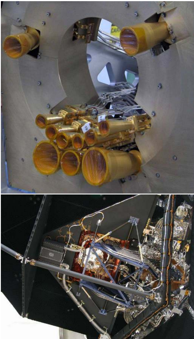
Figure 9. Top panel: picture of the LFI focal plane showing the feedhorns and main frame. The central portion of the main frame is designed to provide the interface to the HFI front-end unit, where the reference loads for the LFI radiometers are located and cooled to 4K. Bottom panel: A back-view of the LFI integrated on the Planck satellite. Visible are the upper sections of the waveguides interfacing the front-end unit, as well as the mechanical support structure.
