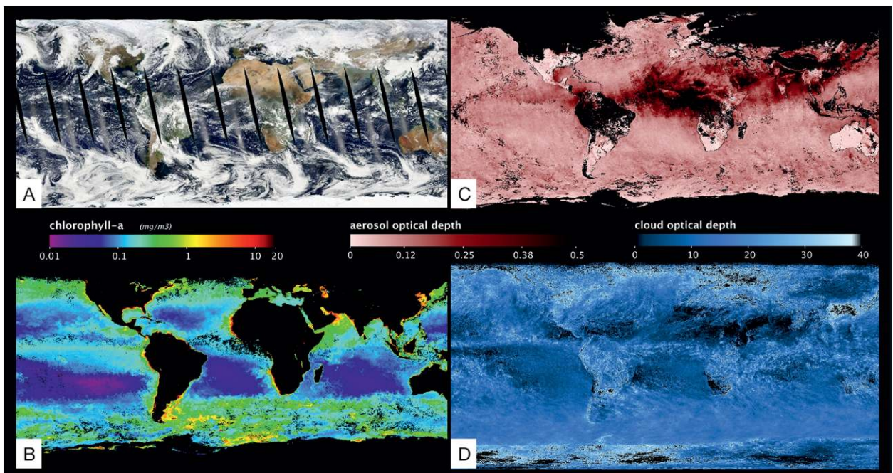
FIG. 1. Example global imagery from MODIS Aqua, representing several data products to be produced by PACE’s ocean color instrument: (a) true color from 10 Jan 2019, (b) average concentrations of chlorophyll a for Jan 2019, (c) average aerosol optical depth for Jan 2019, and (d) average cloud optical depth for Jan 2019. Data acquired from NASA Earth Observations ( https://neo.sci.gsfc.nasa.gov ).
