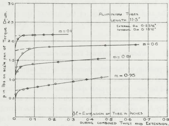
Fig. 6b.—Aluminium Tubes.
