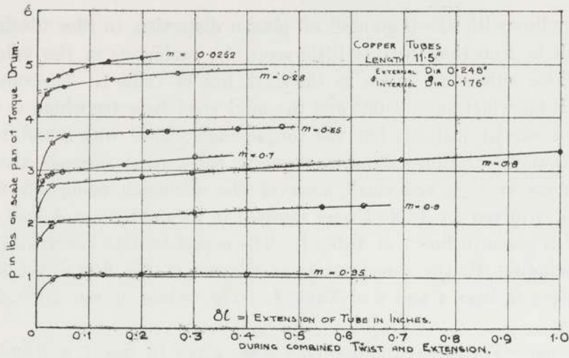
Fig. 6a.—Copper Tubes.
