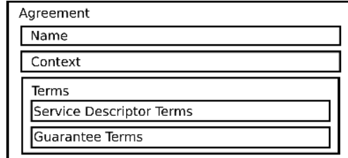
Fig. 6. WS-Agreement Structure
