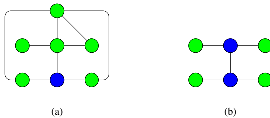
FIG. 5. Minimum covers for (a) a graph G and (b) an induced subgraph of G .
