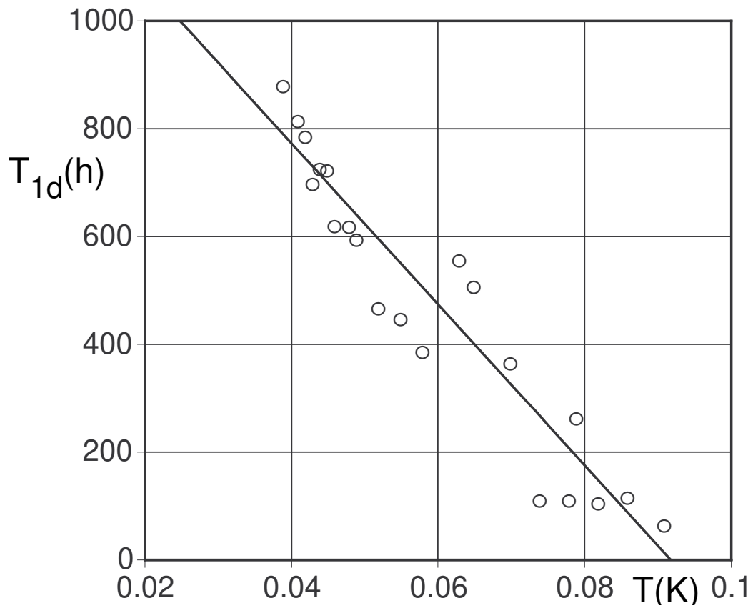
Figure 20: Nuclear spin relaxation times T_{1d}^d in deuterated butanol as a function of temperature T and a magnetic field of 0.5 T.
