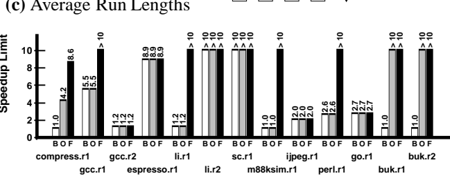
Figure 3. Impact of TLDS on run lengths caused by memory data dependences (B = base case, O = compiler optimizations applied to eliminate dependences, and F = dependences due to forwardable scalars also removed).
