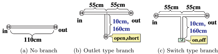
Figure 1. Power line transmission model.
