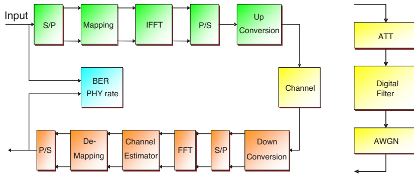
Figure 8. Simulation model of transmission characteristics for OFDM signal using PLC modem.
