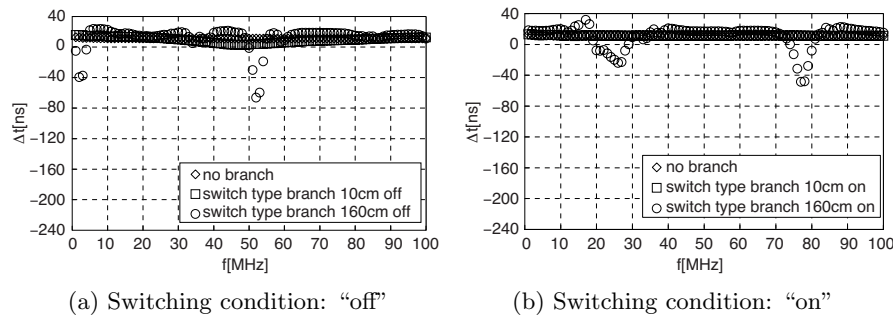
Figure 6. Group delay characteristics of power line (Switch type branch).
