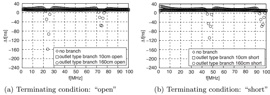
Figure 5. Group delay characteristics of power line (Outlet type branch).
