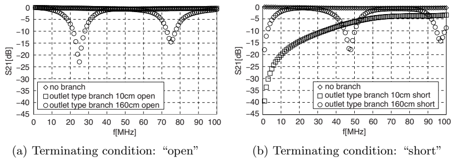
Figure 3. Transmission loss characteristics of power line (Outlet type branch).
