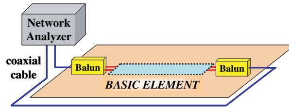
Figure 2. Measurement system of transmission loss characteristic.
