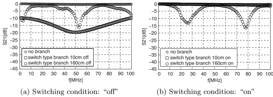
Figure 4. Transmission loss characteristics of power line (Switch type branch).
