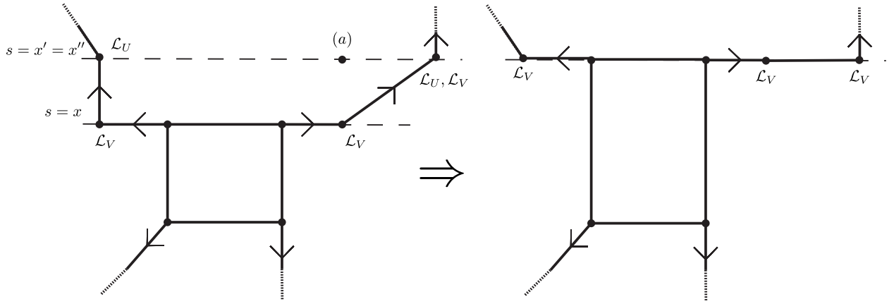
Figure 9: A collapse of two U factors (with identical indices) to a \rho 1_{x'=x''} factor. The point marked (a) indicates the guarded nature of the non-rook move on the right. Note that |\Gamma| - |\Omega| can decrease by at most 1 (and will often stay constant or even increase).
