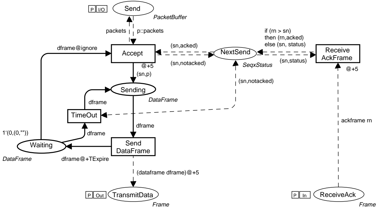
Fig. 25. Timed sender of the stop-and-wait protocol
