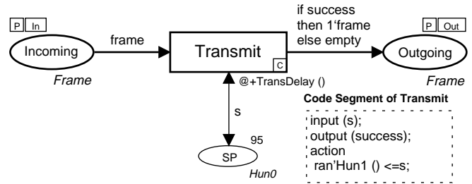
Fig. 27. Timed unidirectional channel
