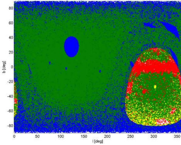
Fig. 24. Sky coverage of the surveys listed in Table 2, in Galactic coordinates. Green points: sources present in both \approx 1 GHz (NVSS or SUMSS) and 4.85 GHz (GB6 or PMN) catalogues; blue points: sources in the NVSS catalogue only; yellow points: sources in the SUMSS catalogue only; red points: sources in the PMN catalogue only; white regions: not covered by any survey.
