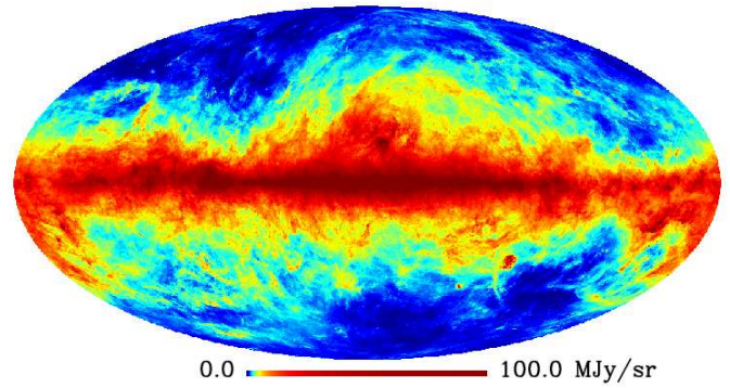
Fig. 13. Map of thermal dust emission 100 \mu\text{m} . Colours are saturated at 100 MJy \text{sr}^{-1} , and the colour scale is histogram-equalised to increase the dynamic range and make both regions of low and high intensity visible.
