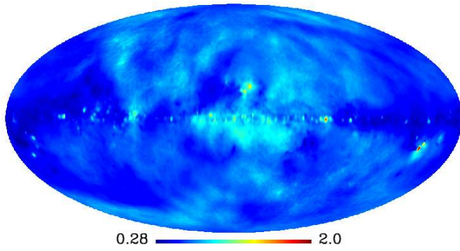
Fig. 12. Map of the ratio of 100 \mu\text{m} to 240 \mu\text{m} emission, as obtained by Finkbeiner et al. (1999) and used in the present model.
