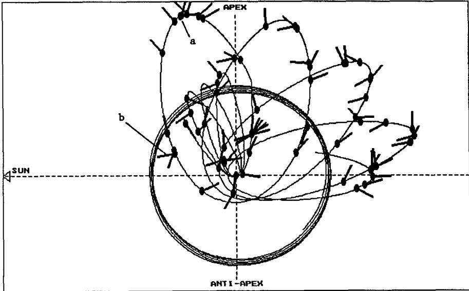
Figure 3. Orbit plot of the HITEN satellite. Positions of dust impact measurements are indicated, the lines show the MDC orientation. A typical apex-particle measurement is marked with "a", a typical beta-meteoroid measurement is marked with "b", see section 5.
