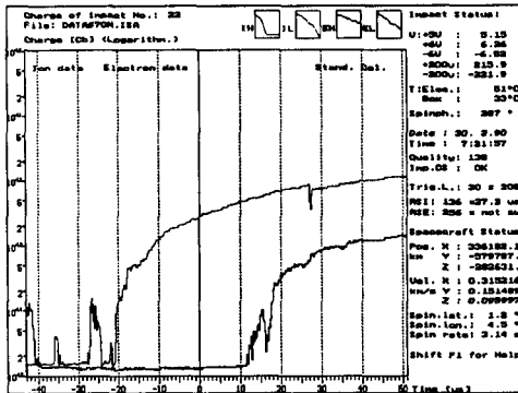
Figure 5a. Typical impact signal of an apex-particle, position of this measurement is marked in fig. 3 with "a".
