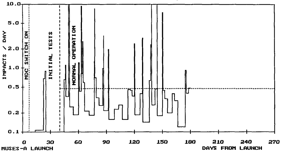
Figure 2. Cosmic dust flux as measured by the MDC in impacts per day
