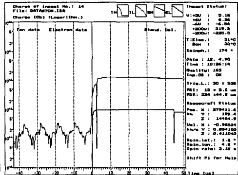
Figure 5b. Typical impact signal of a beta-meteoroid, position of this measurement is marked in fig. 3 with "b".
