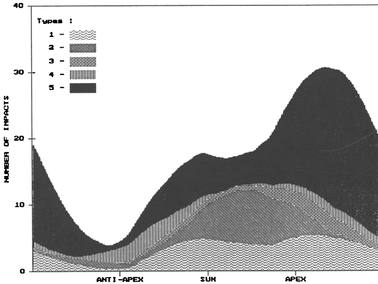
Figure 4. Spin phase angle distribution of dust particles measured by the MDC.
