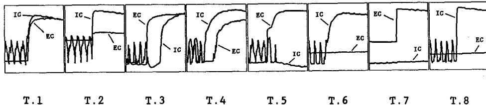
Figure 1. Signal types encountered by the MDC experiment
