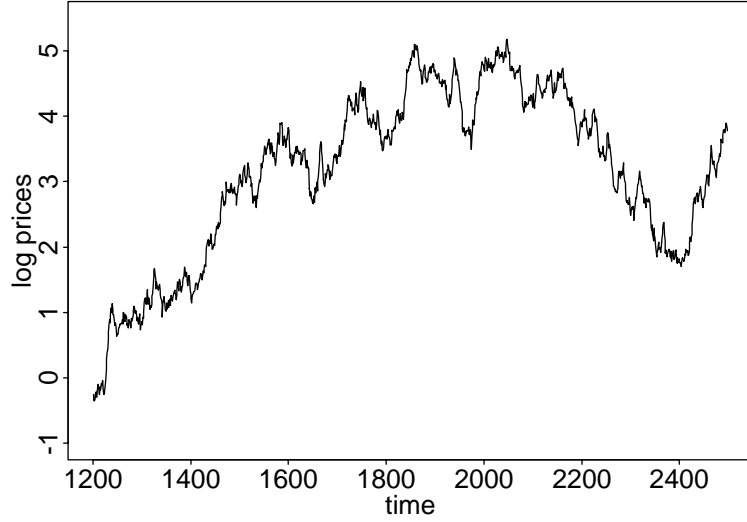
FIGURE 1. Log price vs. time for trend followers with \alpha = 0.2 and \theta = 10 in Equation 10. Trend followers tend to induce short term trends in prices, but they also cause oscillations on longer timescales.
