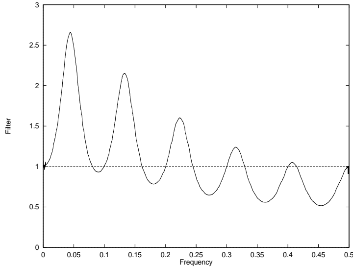
FIGURE 3. Power spectrum of returns induced by a trend following strategy. Same parameters as Figure 2.
