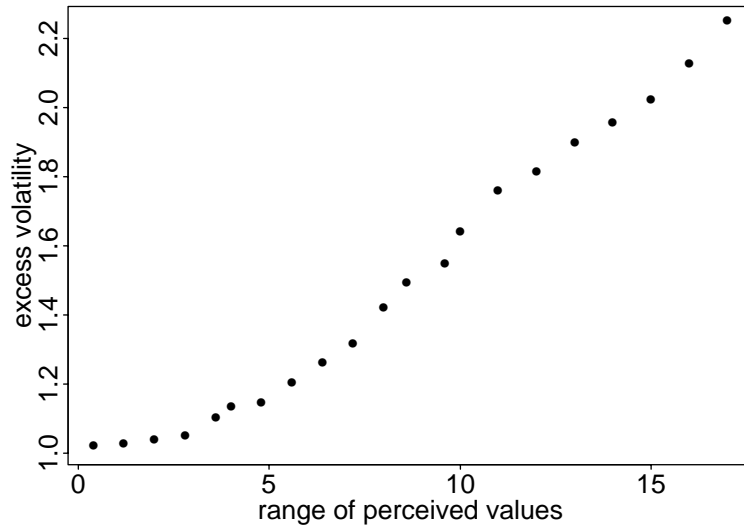
FIGURE 8. Excess volatility as the range of perceived values increases while the capital is fixed at 0.035 . See Equation 19. The other parameters are the same as those in Figure 6.
