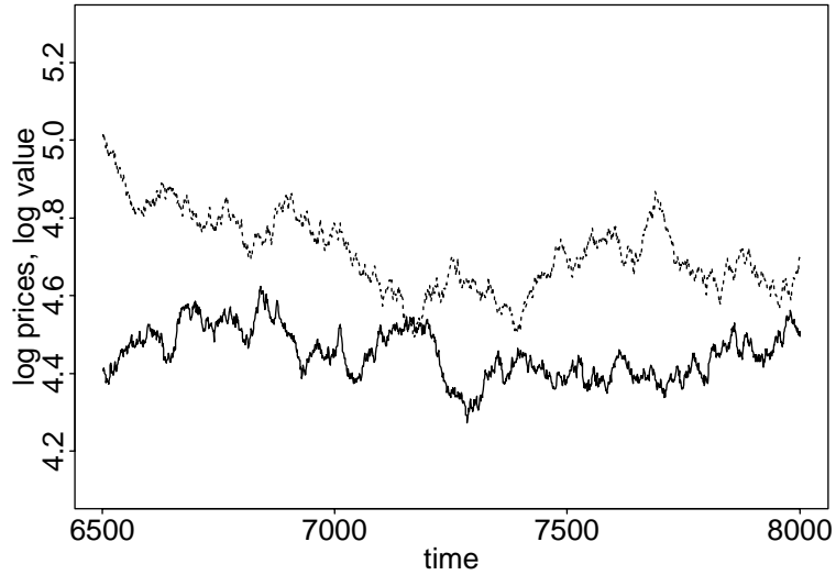
FIGURE 7. Price (solid) and value (dashed) vs. time for the nonlinear state-dependent strategy of Figure 5. The parameters and random number seed are the same as Figure 6, except that \tau_{min} = -0.5 and \tau_{max} = 0.5
