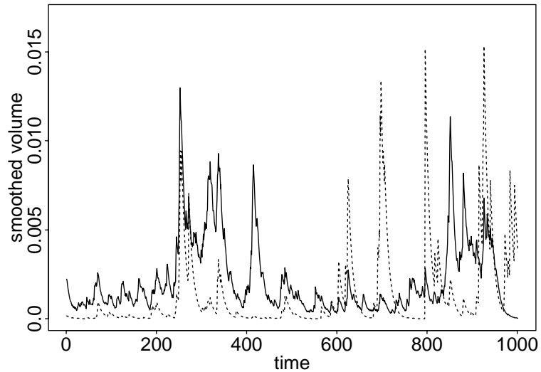
FIGURE 11. Smoothed trading volume of value investors (solid line) and trend followers (dashed line). The two groups become active at different times; when the value investors dominate the log-returns have a negative autocorrelation, and when the trend followers dominate there is a positive autocorrelation. Even though there is no linear temporal structure, there is strong nonlinear structure. Parameters are as described in Table 1; this is only a short portion of the total simulation.
