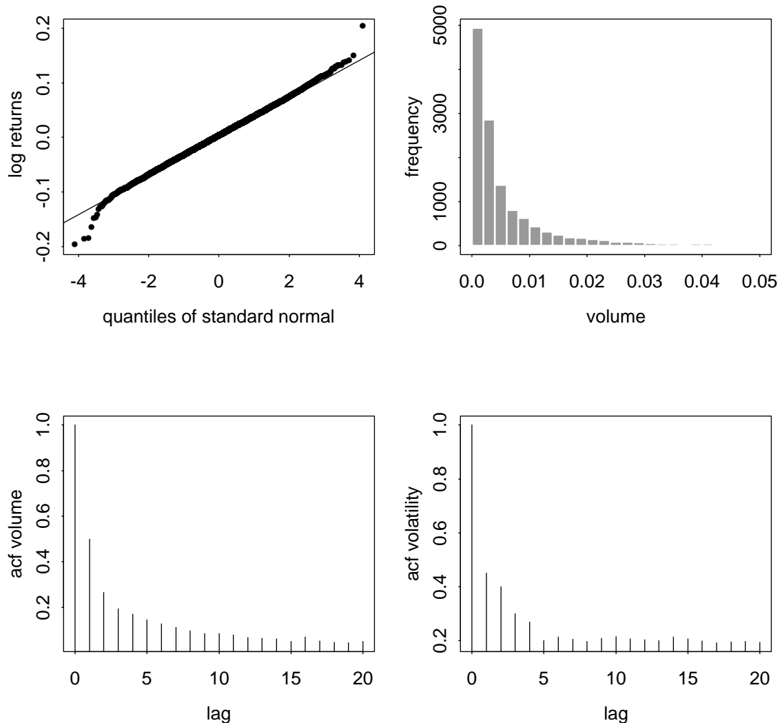
FIGURE 12. An illustration that an ecology of threshold based value investors and trend followers shows statistical properties that are typical of real financial time series. The upper left panel is a “q-q” plot, giving the ratio of the quantiles of the cumulative probability distribution for the log-returns to those of a normal distribution. If the distribution were normal this would be a straight line, but since it is “fat tailed” the slope is flatter in the middle and steeper at the extremes. The upper right panel shows a histogram of the volume. It is heavily positively skewed. The lower left panel shows the autocorrelation of the volume, and the lower right panel shows the autocorrelation of the volatility. These vary based on parameters, but fat tails and temporal autocorrelation of volume and volatility are typical.
