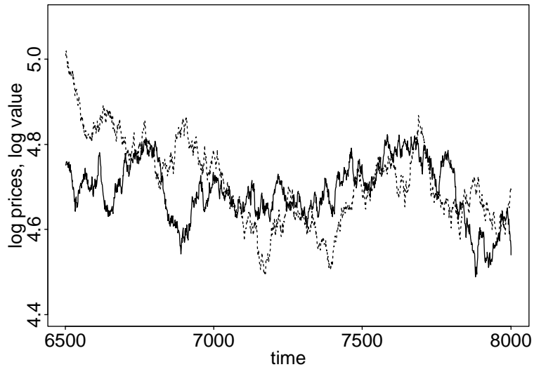
FIGURE 6. The induced price dynamics of a nonlinear state-dependent value strategy with 1000 traders using different thresholds. The log-price is shown as a solid line and the log-value as a dashed line. \tau_{min} = -0.5 , \tau_{max} = 0 , T_{min} = 0.5 , T_{max} = 6 , N = 1000 , a = 0.001 , \sigma_{\eta} = 0.01 , and \sigma_{\xi} = 0.01 , and \lambda = 1 .
