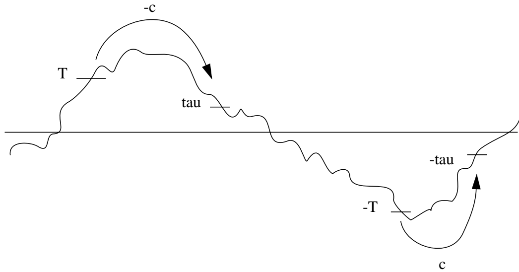
FIGURE 4. Schematic view of a nonlinear, state-dependent value strategy. The trader enters a short position -c when the mispricing m_t = p_t - v_t exceeds a threshold T , and holds it until the mispricing goes below \tau . The reverse is true for long positions.
