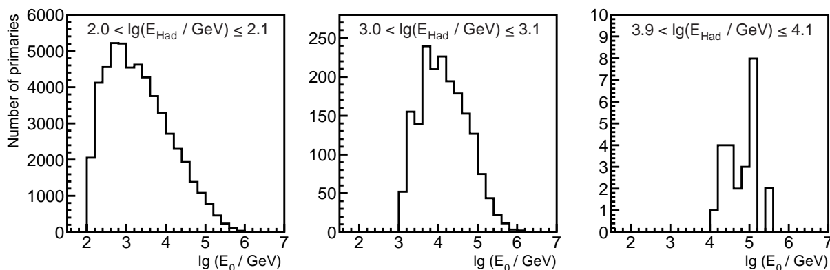
FIG. 5.—Frequency distributions of primary energies for three intervals of single-hadron energies. Simulations with CORSIKA/QGSJET for proton initiated showers are used.
