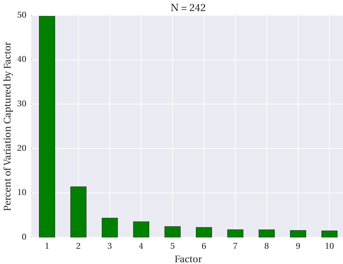
Figure 1: Principal Component Analysis of \widehat{\mathbb{D}}_i Across Firms
