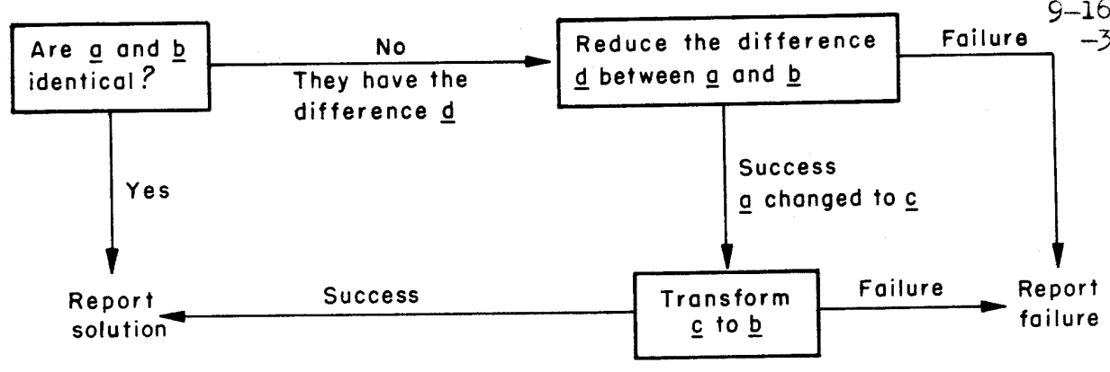
5A—Type 0 goal: Transform a to b
