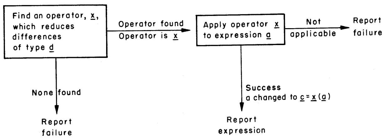
5B—Type 1 goal: Reduce the difference d between a and b
