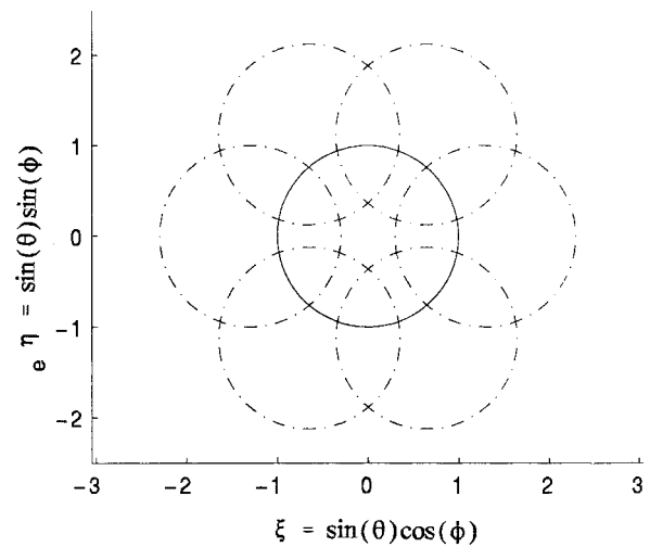
HEXAGONAL SAMPLING ( d=0.89 wavelengths)
