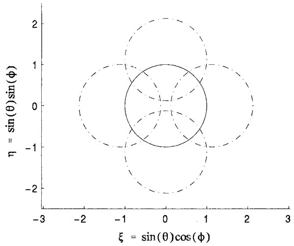
RECTANGULAR SAMPLING ( d=0.89 wavelengths)
